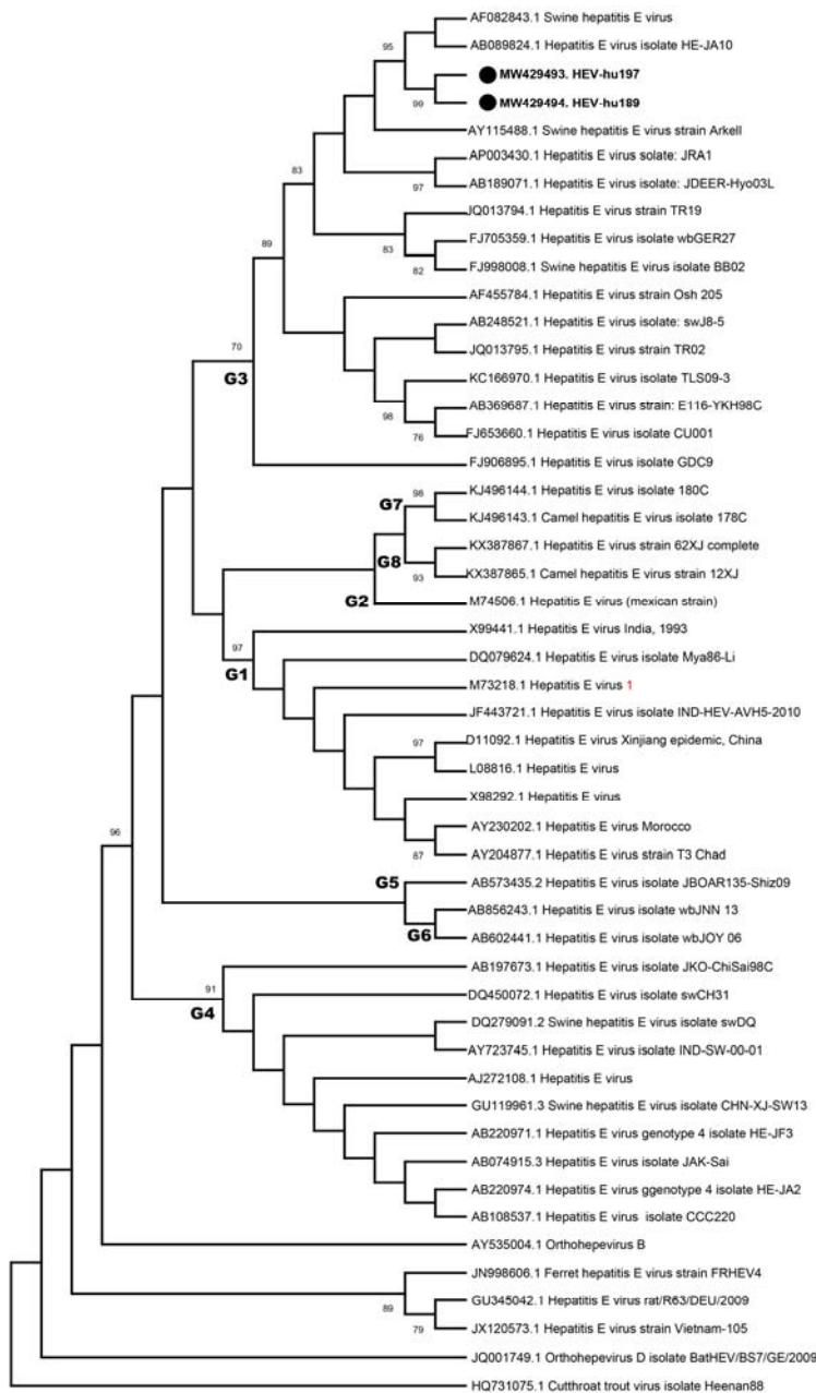
Figure 1. The maximum likelihood analysis of the HEV partial ORF2 sequences (407 nucleotides). The tree is constructed using the General Time Reversible (GTR) model, with a discrete Gamma distribution (+G) for 500 replications. Viruses are indicated by GenBank accession number, name and strain identifier, if available. The sequences characterized in this study are marked and indicated with GenBank accession number. Major HEV genotypes are indicated on the tree. Bootstrap values higher than 70 are provided. Cutthroat trout virus isolate Heenan88 is included as an outgroup.
