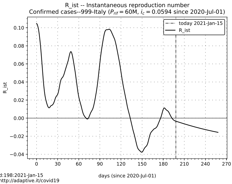
Figure 4: Computed R_{ist} . Fitting model and details at http://adaptive.it/covid19/ [4] data-source: https://github.com/pcm-dpc/COVID-19/ [1]
