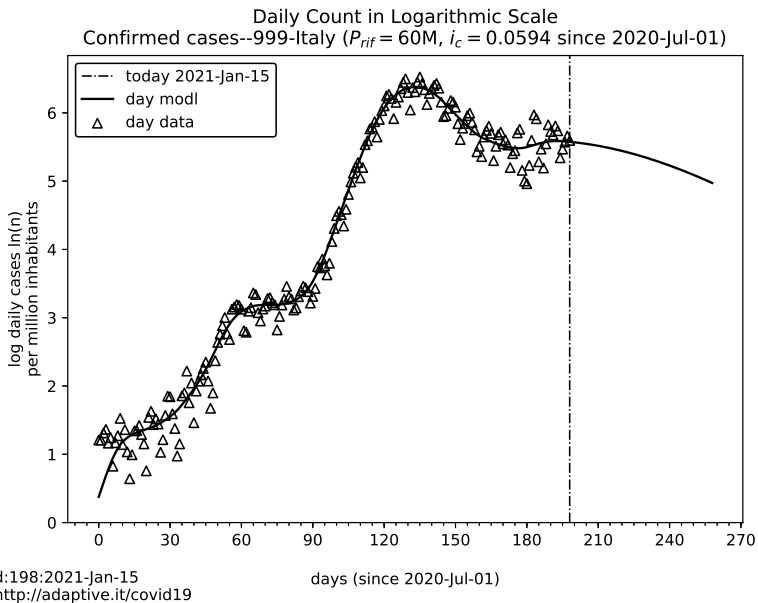
Figure 2: Daily cases smoothed by fitting, in logarithmic scale with base e . Fitting model and details at http://adaptive.it/covid19/ [4] data-source: https://github.com/pcm-dpc/COVID-19/ [1]
