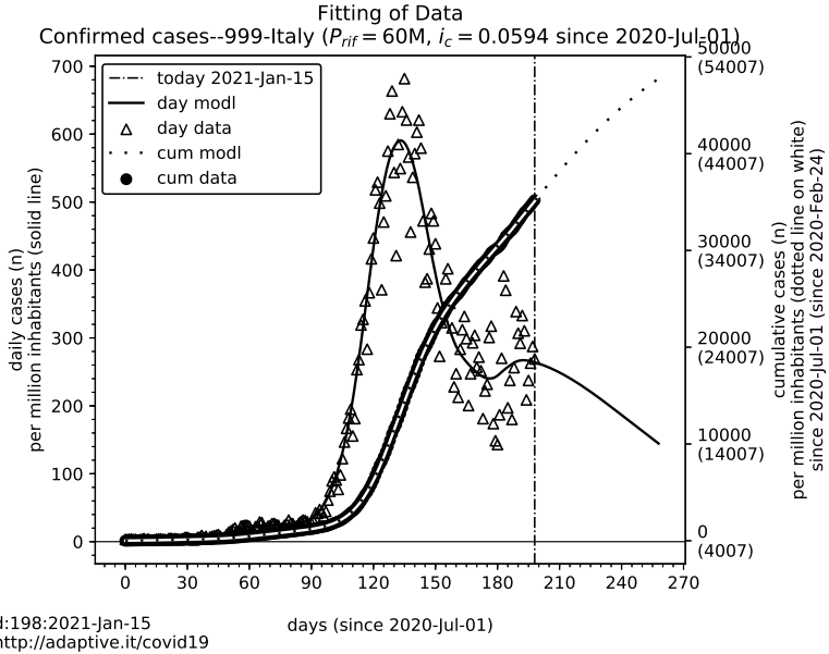
Figure 1: Data fit with an adaptive diffusion/saturation model on cumulative cases. Model and fitting techniques used for these charts are outside the scope of this writing. Fitting model and details at http://adaptive.it/covid19/ [4] data-source: https://github.com/pcm-dpc/COVID-19/ [1]
