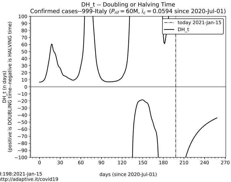
Figure 5: Computed doubling/halving time (days). Negative values mean halving time. Fitting model and details at http://adaptive.it/covid19/ [4] data-source: https://github.com/pcm-dpc/COVID-19/ [1]
