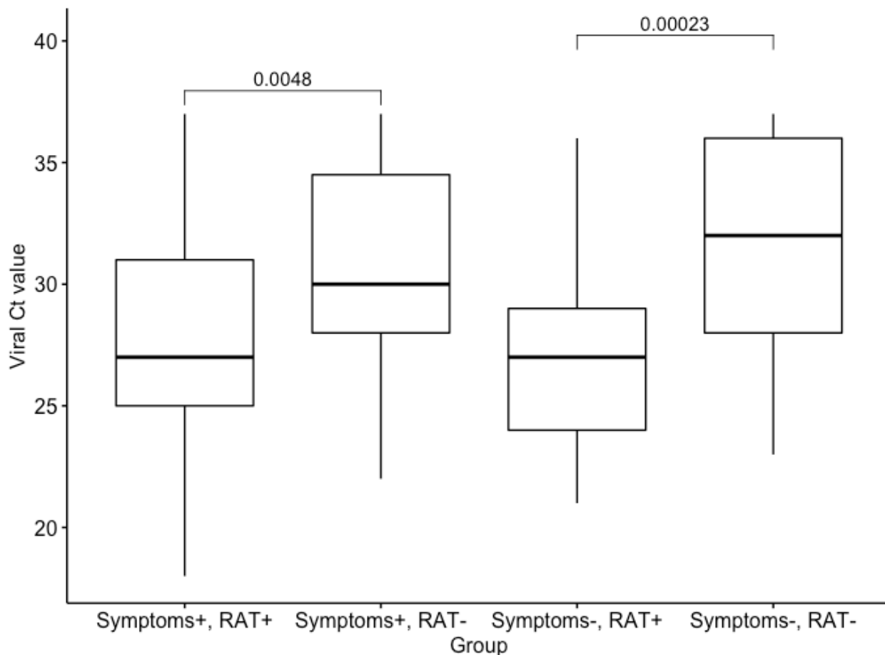
Figure 1: Difference in viral cycle threshold (Ct) value between participants with positive and negative rapid antigen tests among RT-PCR-positive participants with and without self-reported symptoms (n=144). Analysis for statistical difference was performed by Wilcoxon test.
