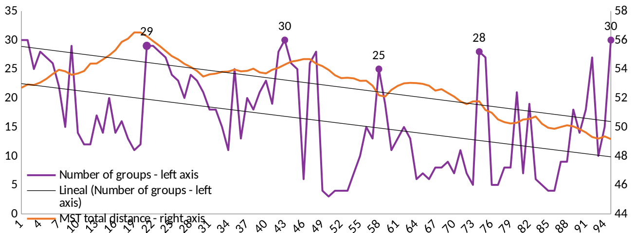
Figure 1: Number of identified groups and MST total distance in each time window
