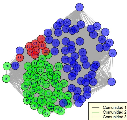
Figure 4. Intensity of similarity in the disease evolution network
