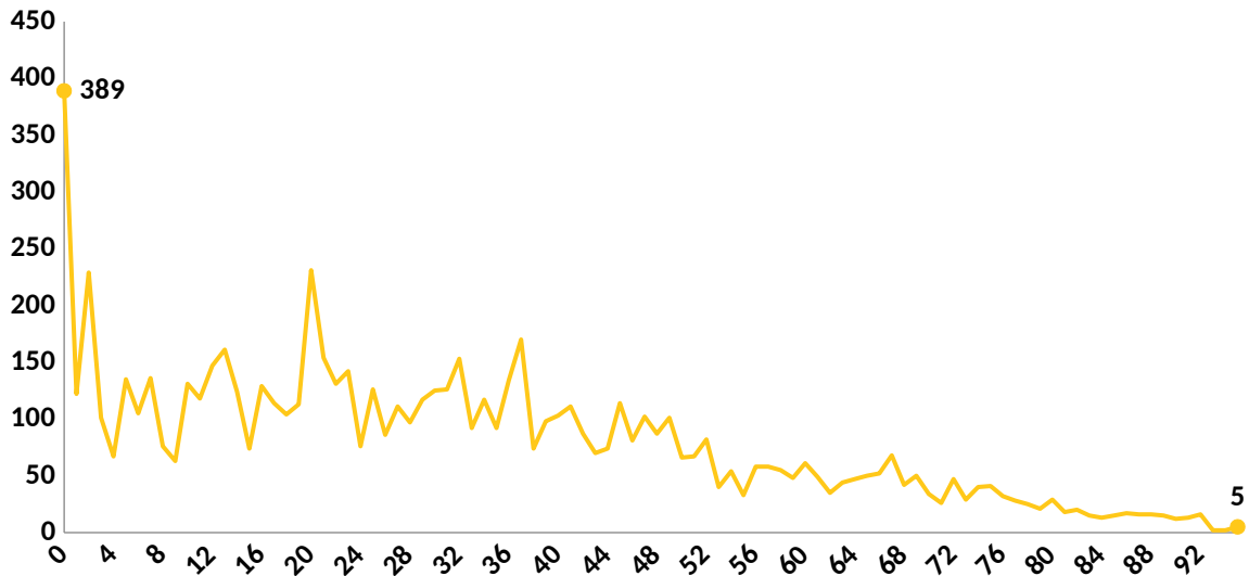
Figure 3: Number of times two countries where in the same group per time window
