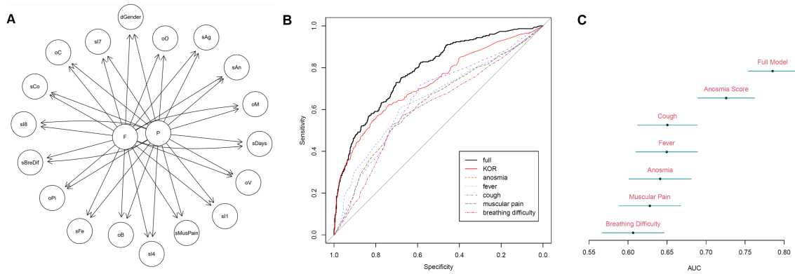
Figure 3: Training of the Bayesian network model for COVID-19 prediction. (A) Structure of the model. P represents the result of the RT-PCR assay, and F represents self-reported cold. The six different odors are represented with the variables: oB (Banana), oC (Caramel), oM (Mint), oO (Orange), oPi (Pineapple), oV (Vanilla). The six different symptoms are represented by: sCo (cough) , sFe (fever), sMusPain (muscular pain), sBreDif (breathing difficulty), sAn (self-reported anosmia) and sAg (self-reported ageusia). Five indicator variables are represented by: sI1, sI4, sI7, sI8, sDays. dGender represents the gender of the individual. All variables are dichotomous. (B) Average Receiver Operating Characteristic (ROC) curve, as estimated through cross-validation ( K = 10 ), for predicting a COVID-19 case using the full model (black line), only the KOR test (red line), and single self-reported symptoms. (C) Mean and 95% confidence intervals for the AUC of the ROC curves shown in (B). These analysis were performed using the UC-Christus sample (N=926)
