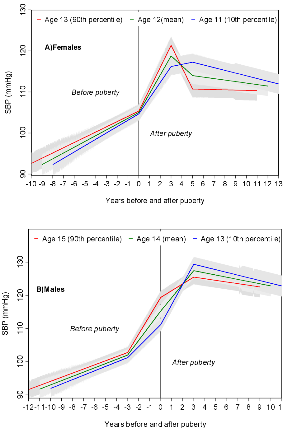
Figure 2 Mean adjusted trajectories of SBP in females and males for the 10 th , median and 90 th sex-specific percentiles of age at peak height velocity from multilevel models based on pubertal age
