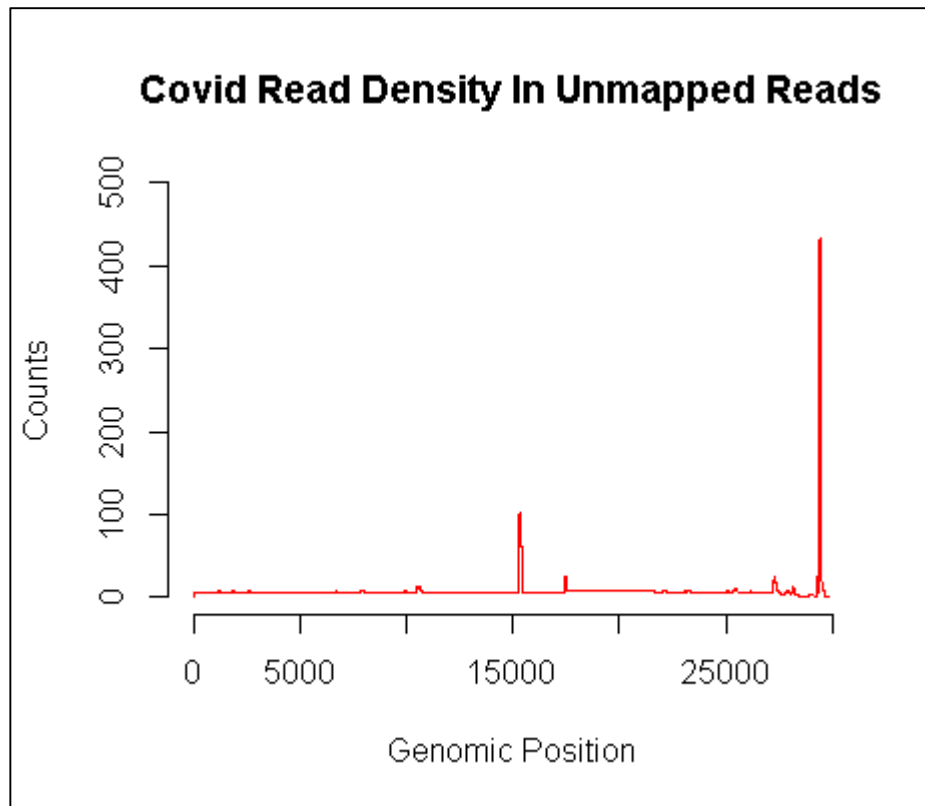
Figure 1: Top panel is the number of reads aligning to the SARS-CoV-2 genome from each patient. Most reads aligned to loci encoding the N protein (red bar) or the RNA dependent RNA polymerase (black bar). Bottom panel is the location where the cumulative reads from all the patients align to the SARS-CoV-2 genome. Genes encoding the RNA dependent RNA polymerase and the N protein are at positions ~15,000 and ~29,000, respectively.
