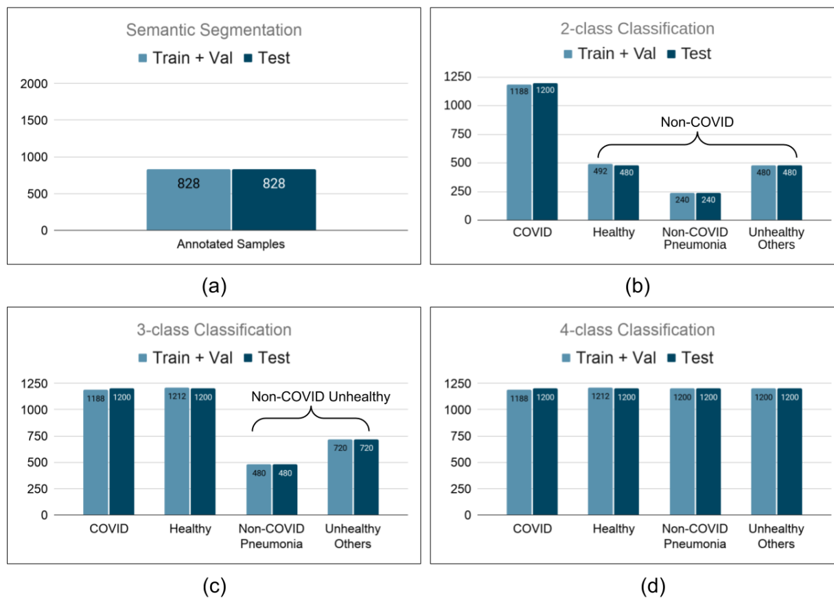
Figure 3. Number of samples present in protocol for (a) Semantic Segmentation. (b) 2-class Classification. (c) 3-class Classification. (d) 4-class Classification.
