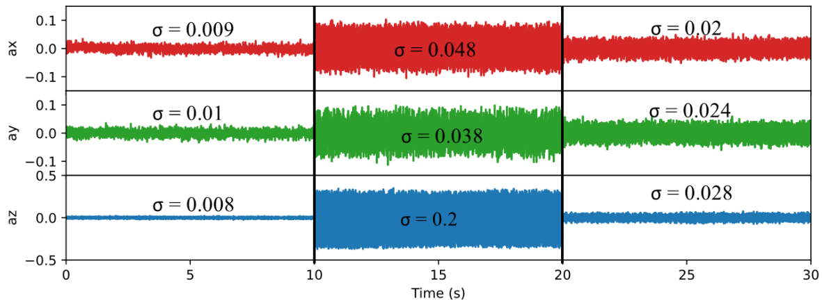
Figure 4: Time variation of accelerometer sensor data from a smartphone placed on the same surface next to the Mobilefuge is plotted to show the vibrations caused by the Mobilefuge. The standard deviation “ \sigma ” of the variation in accelerometer data is shown above for each data set.
