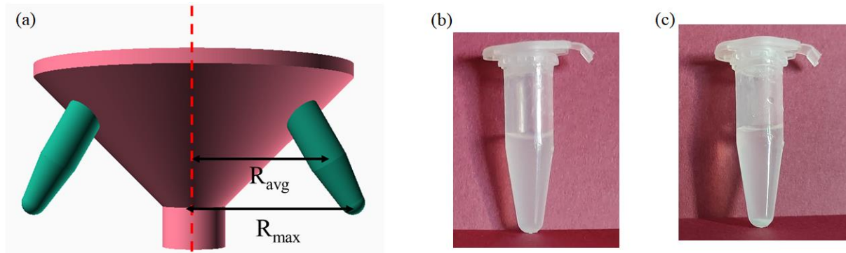
Figure 3: (a) Schematics to show the distance “R” between the rotor and a centrifuge tube used in Eq. (2). (b) “Glass milk” solution with silica particles in a 2mL centrifuge before the centrifugation (c) Pellet of silica particles formed after centrifugation of the “glass milk” solution with Mobilefuge for 30 seconds.
