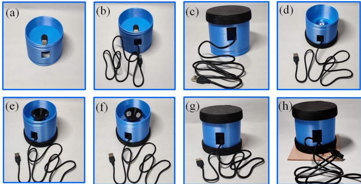
Figure 2: Assembly instructions of the Mobilefuge: (a) Fan motor is press-fitted at the bottom of the jar (b) A USB cable is connected to the motor (c) Bottom lid is fixed to the jar part of the enclosure. (d) Same as (c) but showing the top view of the jar with the bottom lid in place (e) Rotor is press-fitted to the fan motor (f) Centrifuge tubes inserted in the rotor (g) Top lid is threaded to the main jar of the enclosure to complete the assembly of the Mobilefuge. (h) A self-adhesive damping pad is placed at the bottom of the Mobilefuge to improve the stability of Mobilefuge.
