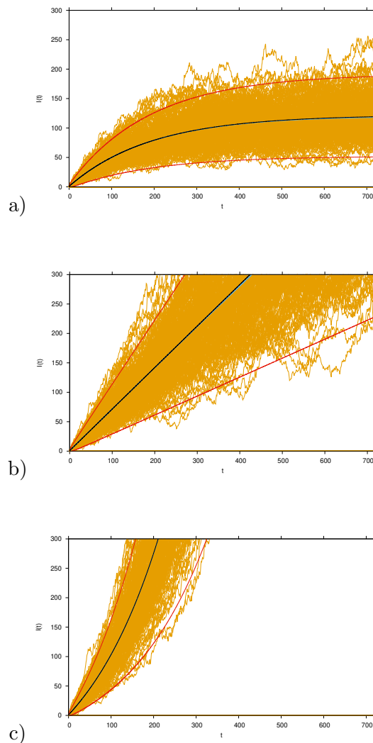
Figure 2: Mean dynamics and variance curves ( \mu \pm 2\sigma ) and stochastic realizations of SIR model with import. Increased import \varrho = e^{-12} . Variation of \beta with a) \beta = 0.9 \cdot \gamma , b) \beta = \beta_c = \gamma and c) \beta = 1.1 \cdot \gamma .
