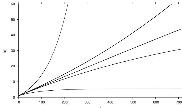
Figure 3: For community infectivity very close to criticality \beta = 0.99 \cdot \gamma and \beta = 1.01 \cdot \gamma the solutions appear initially close to the critical line of \beta = \beta_c = \gamma , but finally level off subcritically again, respectively explode into the exponential phase. Analytic mean field solution from bottom to top for \beta = 0.9 \cdot \gamma , \beta = 0.99 \cdot \gamma , \beta = \beta_c = \gamma , \beta = 1.01 \cdot \gamma and \beta = 1.1 \cdot \gamma , in all cases import \varrho = e^{-15} and N = 2 \cdot 10^6 and \gamma = 0.05 d^{-1} .
