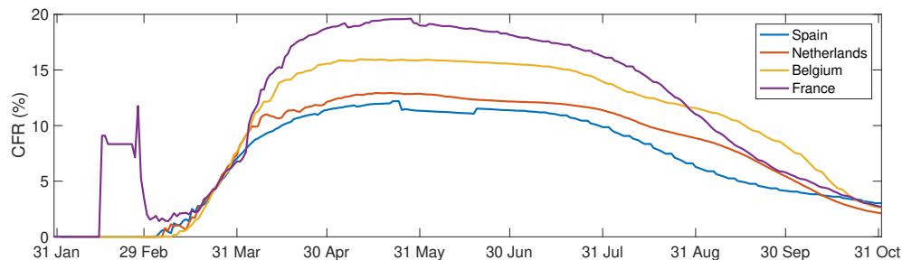
Figure 15: Evolution of the case-fatality ratio for Spain, the Netherlands, Belgium, and France until the end of October 2020.
