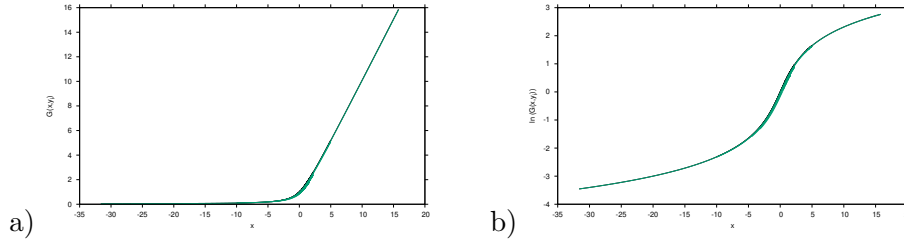
Figure 10: a) Scaling function G(x, y = 1) = x/2 + \sqrt{x^2/4 + y} , and data collapse of the stationary state density I^*/N for \varrho_1 = 0.1 , \varrho_2 = 0.05 , \varrho_3 = 0.01 and \varrho_4 = 0.001 , and \varepsilon varied from \varepsilon = -0.5 to \varepsilon = 1 , hence \beta = \gamma + \varepsilon varies from \beta = 0.5 to \beta = 2 . b) Same for \ln(G) . In both cases we use x := a_\varepsilon \varepsilon (a_\varrho \varrho_i)^{-1/\hat{\sigma}} and y := \ln \left( (a_\varrho \varrho_i)^{-\hat{\beta}/\hat{\sigma}} \cdot \frac{I^*}{N}(\varepsilon, \varrho_i) \right) with \frac{I^*}{N} = \frac{1}{2\beta} (\beta - \gamma - \beta\varrho) + \sqrt{\frac{1}{4\beta^2} (\beta - \gamma - \beta\varrho)^2 + \varrho} and a_\varepsilon = 1/\beta and a_\varrho = 1 , \hat{\beta} = 1 and \hat{\sigma} = 2 . Here we simply use \gamma = 1 , hence time scales with inverse recovery rate.
