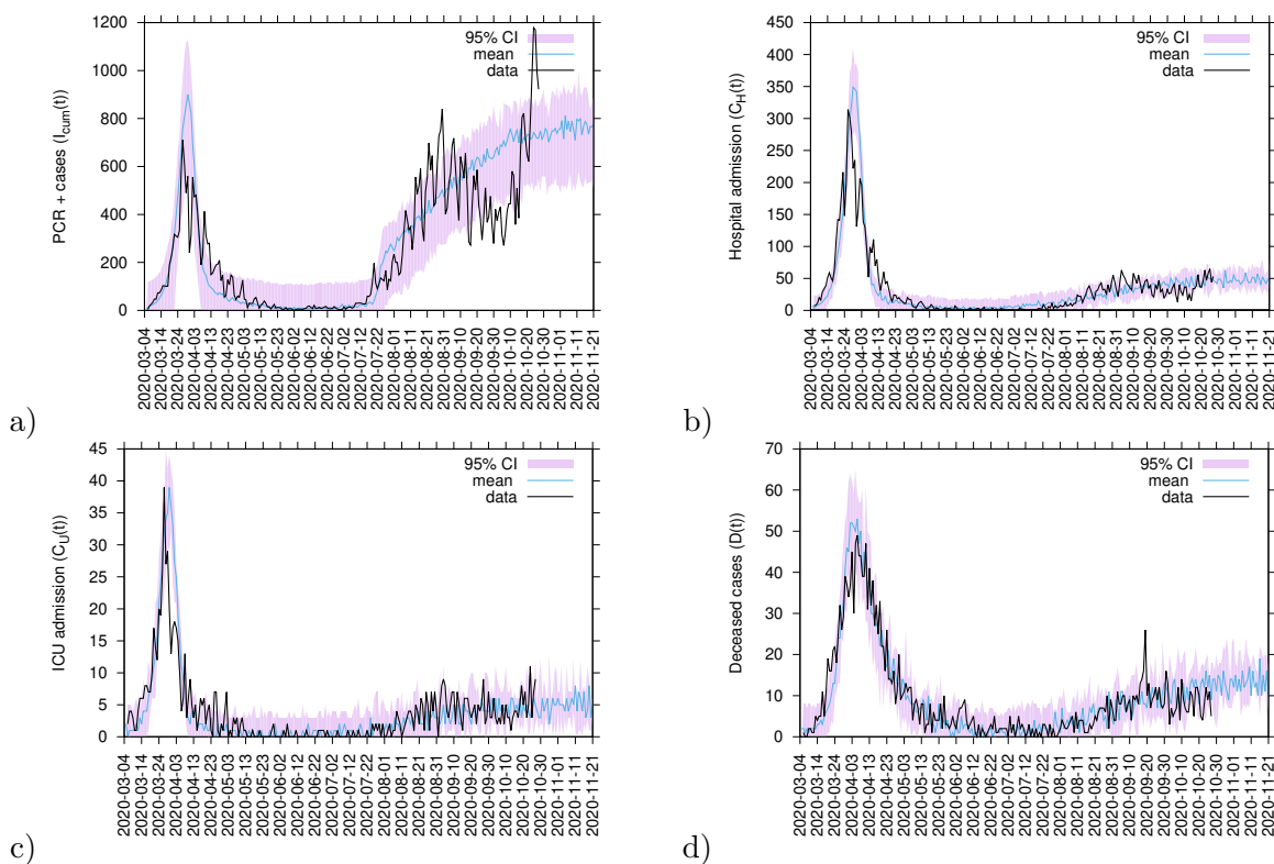
Figure 7: Incidences updated for a) positive tested, b) hospitalized, c) ICU admitted and d) deceased cases, until end of October 2020. Here we see the initial increase to a second phase, of disease spreading from late July and August 2020 on, so called “second wave”, but then the leveling off to a stochastic fluctuating stationary behaviour.
