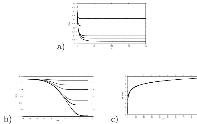
Figure 12: For vanishing distance to criticality \varepsilon = 0 we have the time dependence a) in natural scale b) in double logarithmic scale and in c) as scaling of data collapse.
