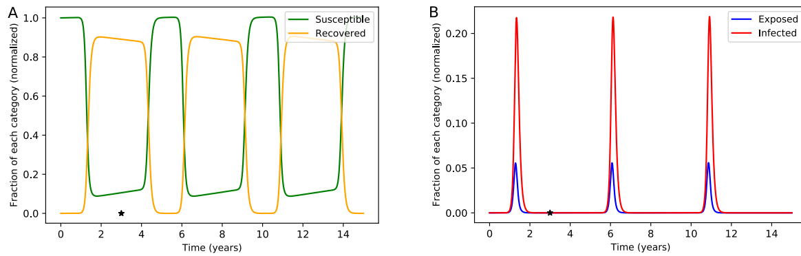
Figure 2) Retarded SEIRS Model for COVID-19 epidemics. A) S and R proportions. B) E and I proportions. Both figures are for one simulation, and are drawn in two parts because of better representation. Here it is assumed that each recovered individual is immune for T = 3.0 years. So at t = 3.0 years and after that, the immunity of individuals who got infected early in the outbreak will be lost. The asterisk shows the first individual who loses the immunity, which corresponds the first infected individual. After the first peak of the epidemic, the proportion of E and I will decrease sharply and then increase again. Epidemics occur every few years, approximately every five years. It should be noted that each of E and I proportions sometimes fall below 10^{-12} —for example, between the first and second epidemic peaks—and these events cannot be observed in human societies. This simulation shows that the use of numerical methods, regardless of the S , E , I and R values, can lead to unrealistic results. The parameters used in this simulation are are shown in table 1. To view the code related to this simulation, refer to SEIRS.Figure.2.py code (supplemental files).
