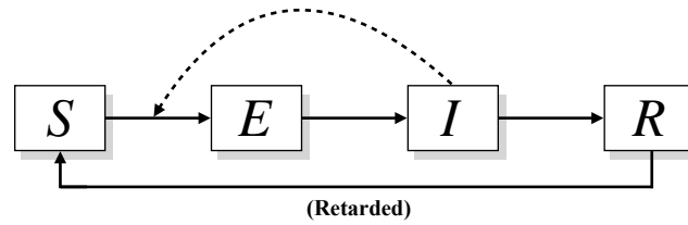
Figure 1) Retarded SEIRS model overview. Susceptible individuals will be exposed by infected individuals. Exposed individuals will then enter the infected category after a short time. The infected individuals will recover, and then join the susceptible category again. It should be noted that for better understanding, births and deaths are not included in this figure. But it is clear that the births should be included in some categories; in addition, given that natural death occurs in all categories, another output must be considered for each category. Also, some individuals will die in the infected category due to the fatality of the disease.
