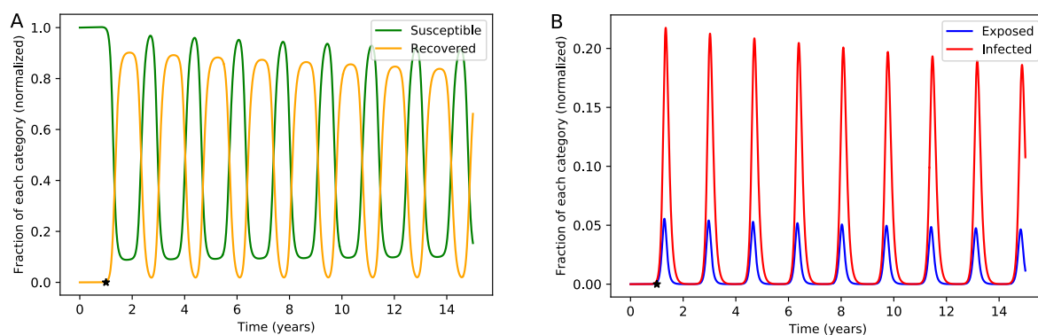
Figure 3) Simulation of Retarded SEIRS model, for T = 1.0 years over fifteen years. A) S and R proportions. B) E and I proportions. It is emphasized again that both diagrams are related to one simulation and are calculated for one-year temporary immunity duration. The other parameters are the same as the parameters in table 1. The first, second, and third epidemics (and even after them) can be clearly seen from the curve of I (or other categories). To view the code related to this simulation, refer to Retarded .SEIRS .Figure.3.py code (supplemental files).
