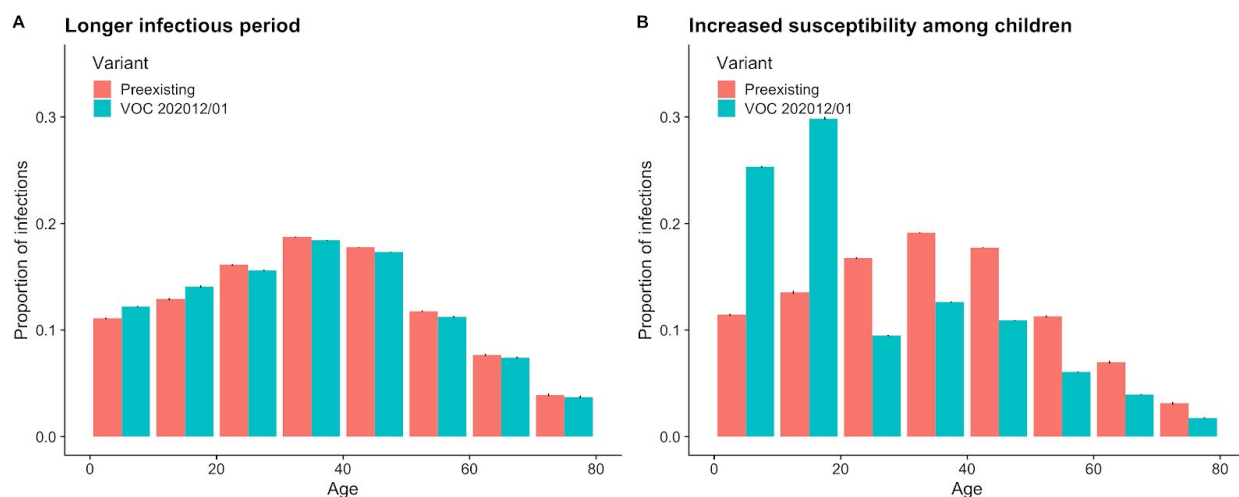
Fig. S16. Comparison of age distribution of infections in the two-strain model depending upon biological mechanism of VOC 202012/01 growth rate. Contrasting (A) longer infectious period and (B) increased susceptibility among children models. Measured from infections in the fitted model between 1 November and 15 December 2020 in the South East NHS region..
