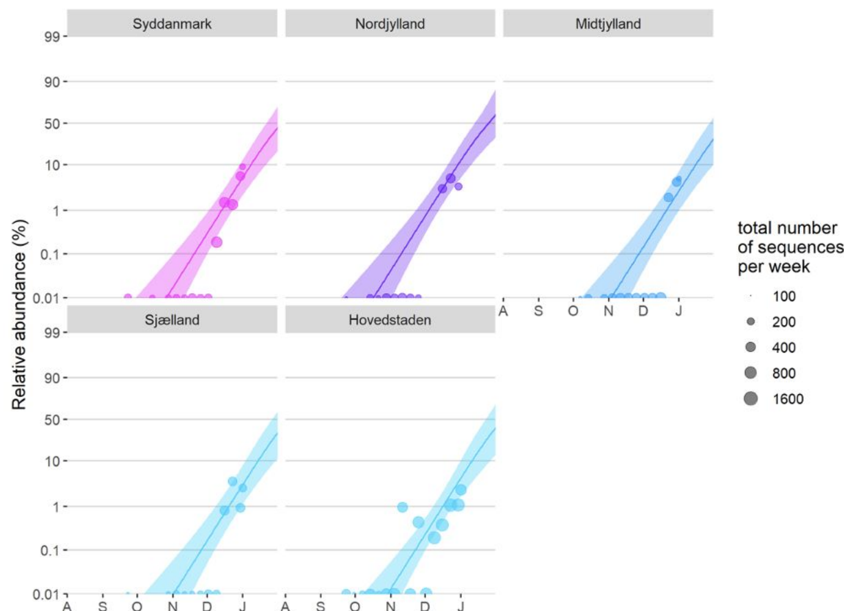
Fig. S6. Independent estimate of the rate at which VOC 202012/01 is displacing other variants based on the random sequencing of SARS-CoV2 strains in Denmark, reported on an aggregated per-week basis (56) (for week 39 of 2020 until week 1 of 2021). A binomial GLMM with a common slope across regions and an observation-level random effect to take into account overdispersion fitted the data best, based on the BIC criterion, and resulted in an estimated selection rate \Delta r of 0.10 [0.07, 0.12] 95% CIs (Table S1, model 3a). In addition, a model with separate slopes per region showed that there were no significant differences in the slopes and implied rates of spread across regions (pairwise Tukey posthoc tests for differences in slope, all P > 0.05 ).
