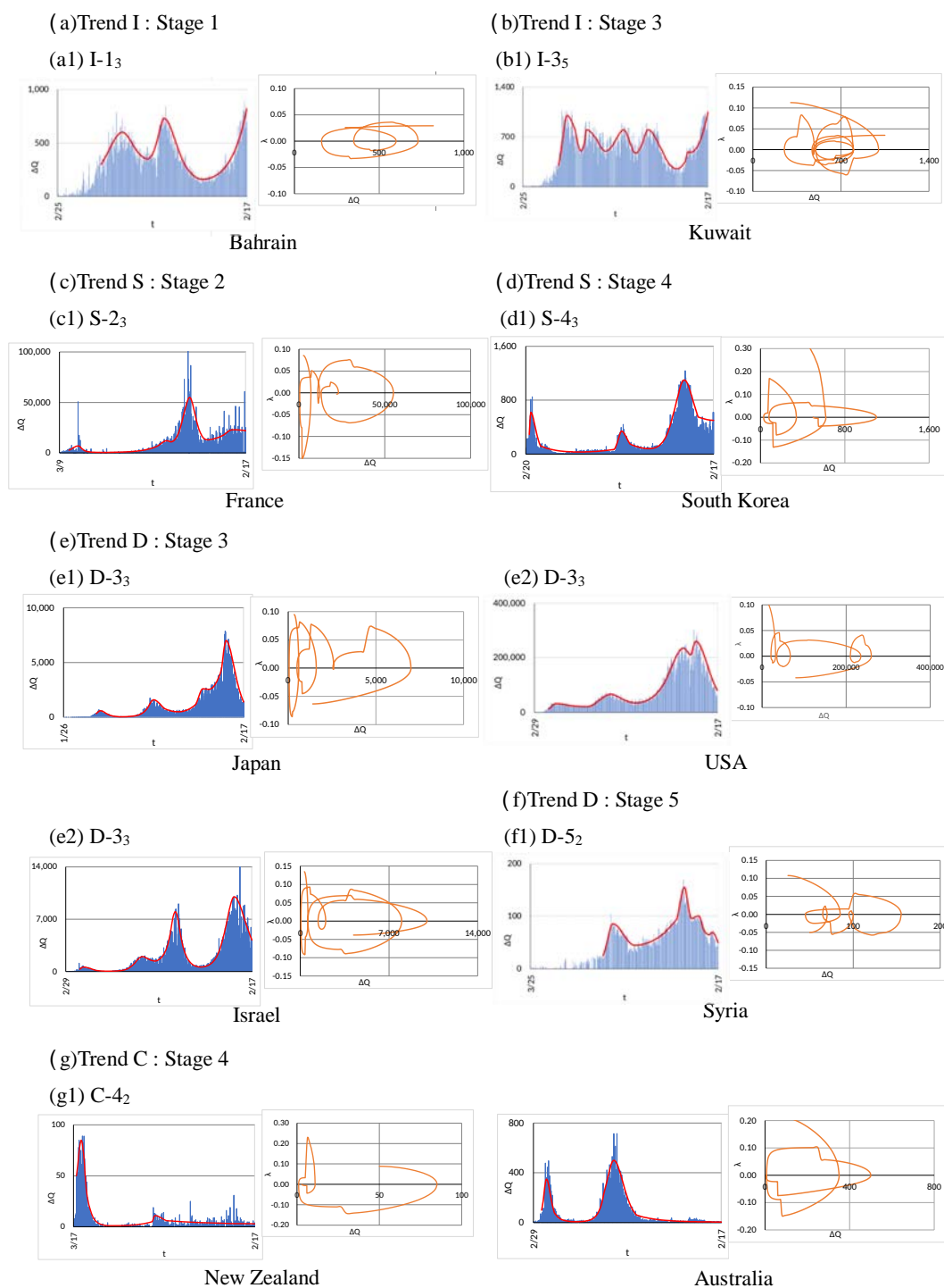
Figure 2: Infection curves from January 23, 2020 to February 17, 2021 for ten countries in different trends: (a) and (b) increasing trend, (c) and (d) stationary trend, (e) and (f) decreasing trend and (g) converged. See the following section for the classification scheme. In each country, the panel on the left hand side is the infection curve \Delta Q(t) with fitting by Eq. (1), and the panel on the right hand side in each country is the infection status plot, \lambda vs \Delta Q . Note differences in the scale of axes. Data from Coronavirus Resource Center, Johns Hopkins University [1].
