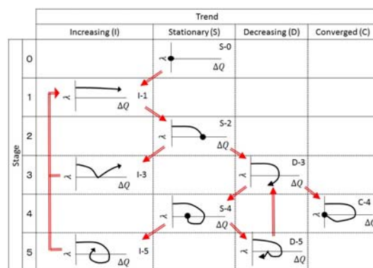
Figure 3: Classification of infection status by the infection status plot. Solid circles denote that the plot is stationary. Red arrows indicate the direction of the possible change of the states. I-3 and I-5 are equivalent to I-1, and D-5 is equivalent to D-3.
