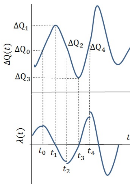
Figure 1: Setting of parameters for an infection curve. In each time period, \lambda(t) is approximated by a quadratic function shown in Table 1.
