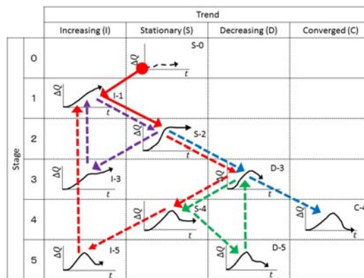
Figure 4: The infection curves for different infection states. The solid red arrows indicate the process of outbreak in most of the countries. Red dashed-arrows are the trajectory of a wavy infection and blue dashed-arrows indicate an efficient conversion process. Step-wise increase and step-wise decrease are denoted by purple dashed-arrows and green dashed-arrows, respectively.
