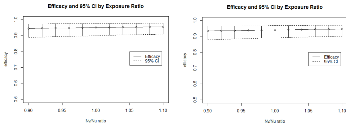
Figure S1. Efficacy and 95% confidence interval by varying exposure ratio. Left panel: Pfizer-BioNTech vaccine; Right panel: Moderna vaccine
