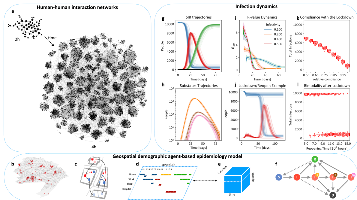
Fig. 1: The nonlinear network effects of SARS-Cov-2 outbreaks are quantified with non-homogenous spatio-temporal models of individual human behavior. a, Human-human interactions create dynamic stochastic networks in space and time. b, The model uses data from real-world communities with annotated buildings, demographics, and statistics on daily occupations ( Movie 1 ). c, Individuals move between locations to meet other individuals, enabling infection transmission. d, Schedules define typical behavior and whereabouts of individuals per hour. e, Individuals, locations, and time span a multidimensional space for stochastic simulations. f, An individual's health status can be susceptible - S, infected - I, recovered - R, deceased - D, and infection sub-states a- or presymptomatic (plain I), diagnosed ( I^d ), hospitalized ( I^d_H ), in intensive care ( I^d_{ICU} ). g, Simulation of uncontrolled baseline scenario for a town (here the German town Gangelt with 10.351 individuals), starting from 4 infected individuals; dynamics of states S, I, R, and D over approx. 12 weeks (100 replicates, colors as in f ). h, Dynamics of I, I^d , I^d_H , and I^d_{ICU} (colors as in f ). i, The R-value as emergent model property for different values of the model parameter infectivity, which may change with NPIs such as mask wearing or social distancing. j,
