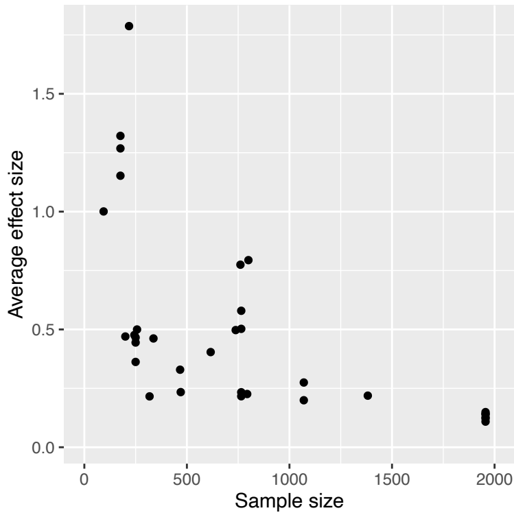
898 Figure S2. Relationship between study sample size and average extracted effect size 899 across all studies.
