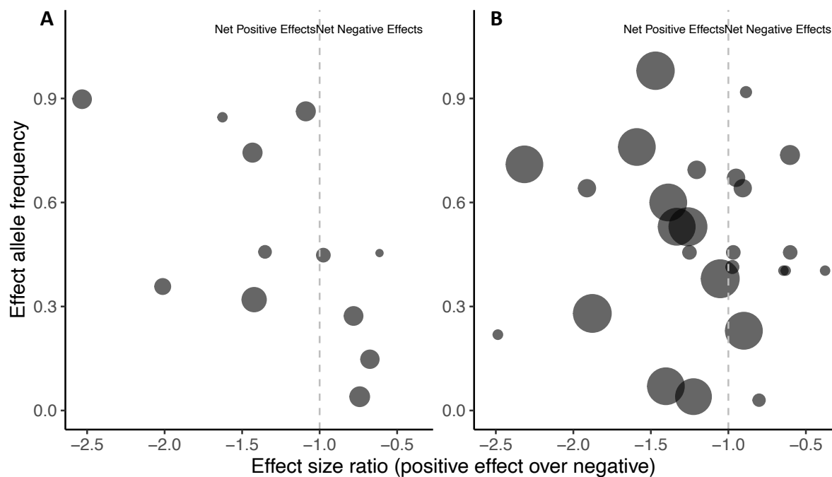
910 Figure S4. The relationship between effect allele frequency and effect size ratio, grouped 911 by trait class. Points to the right of the vertical dotted line have a greater negative effect than 912 positive. A. Disease risk/severity variants. B. Complex traits. Point size is based on the variance 913 of the effect size ratio, with smaller variance having larger point sizes and greater weighting 914 in the statistical model.
