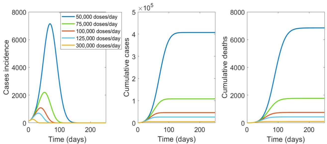
Figure 2: The impact of speed of mass vaccination with a vaccine of 90% efficacy. From left to right is the epidemic curve, the cumulative case and deaths numbers by number of number of people vaccinated per day in NSW.
