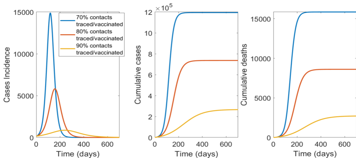
Figure 4: The impact of contact tracing and ring vaccination on epidemic control for a vaccine with 45% efficacy as post-exposure prophylaxis: From left to right is the epidemic curve, the cumulative case and deaths numbers by percentage of contacts traced and vaccinated
