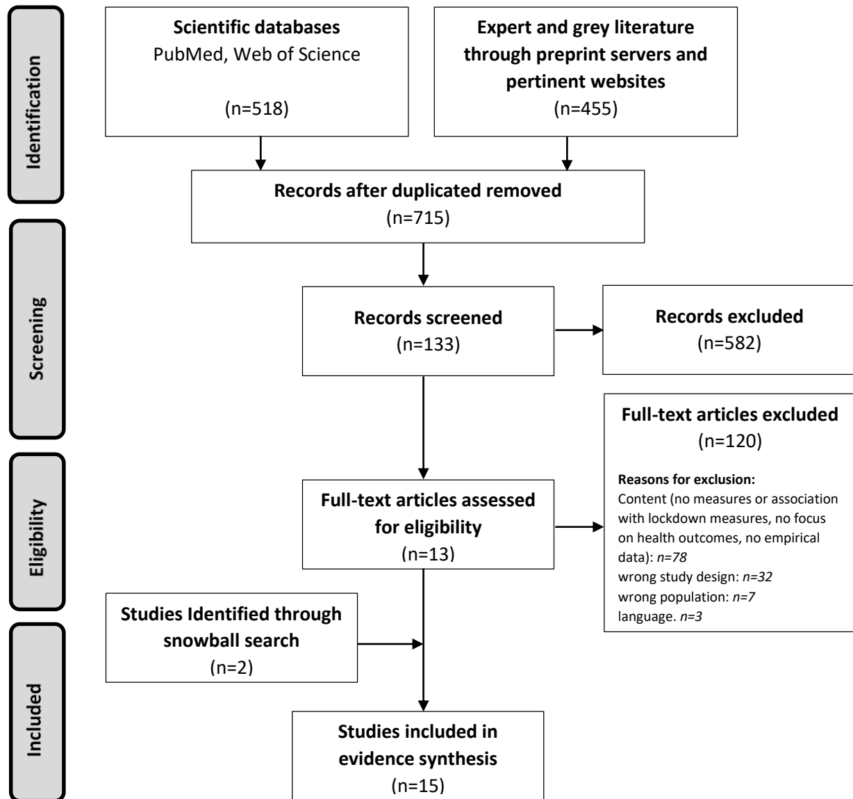
Figure 2: PRISMA Flow-Chart
