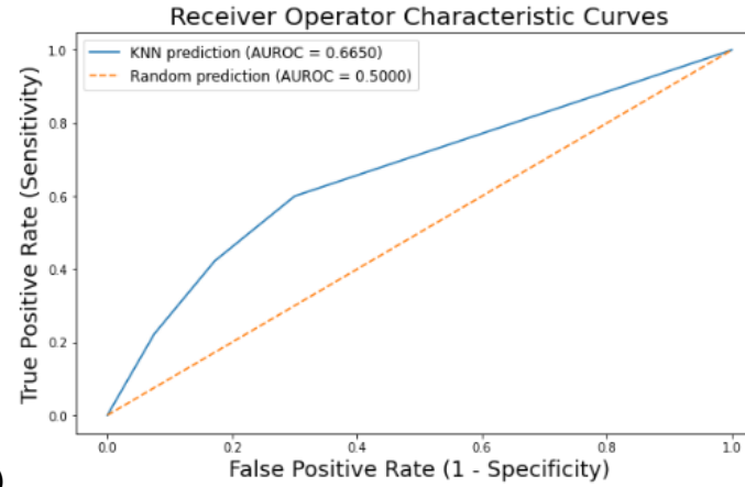
Supplemental Figure 1. Receiver Operating Curve with AUROC for a) RF, b) kNN, c) SVC-RBF, d) DT, e) ABC , f) QDA and g) Deep-FLAIM
