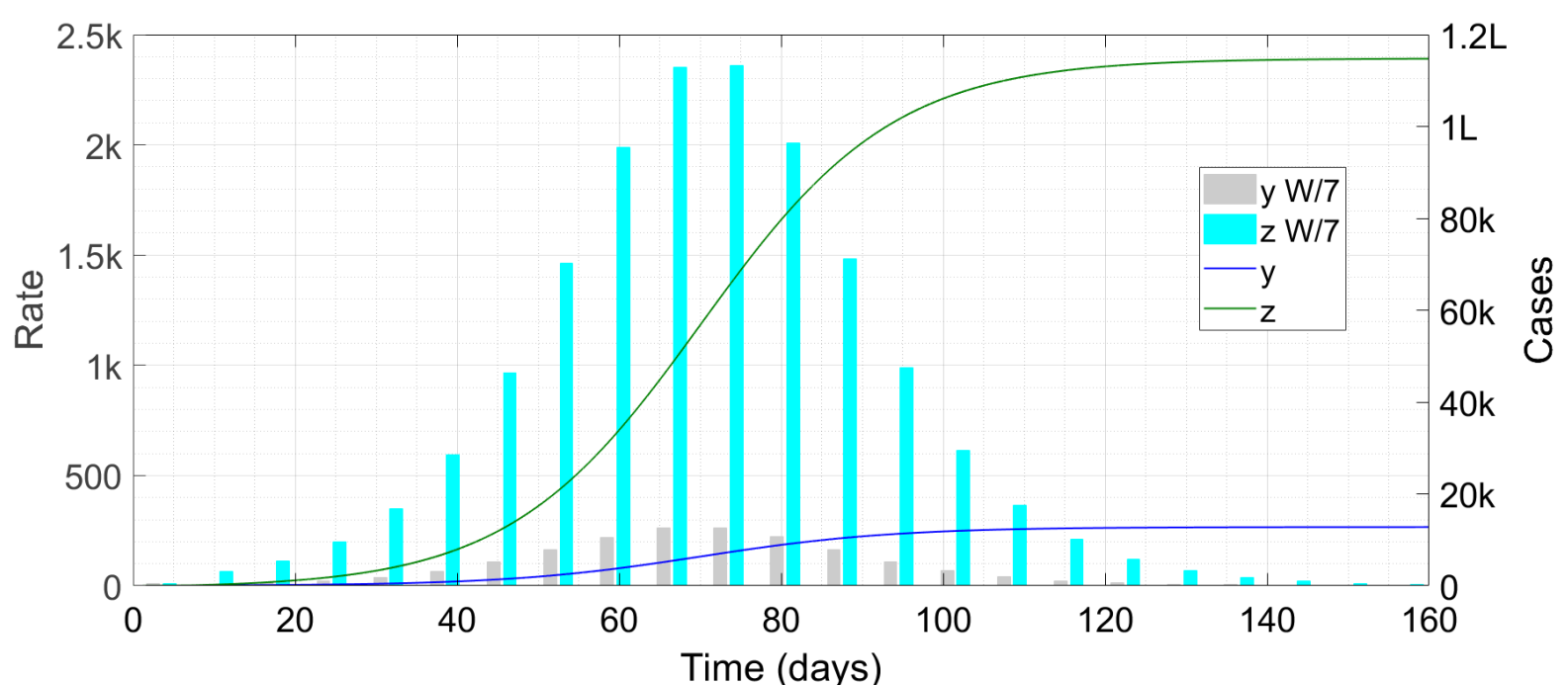
Figure 1 : Time trace of the epidemic without vaccination. The symbol ‘k’ denotes thousand, ‘L’ hundred thousand and ‘W/7’ weekly cases scaled down by a factor of seven.
