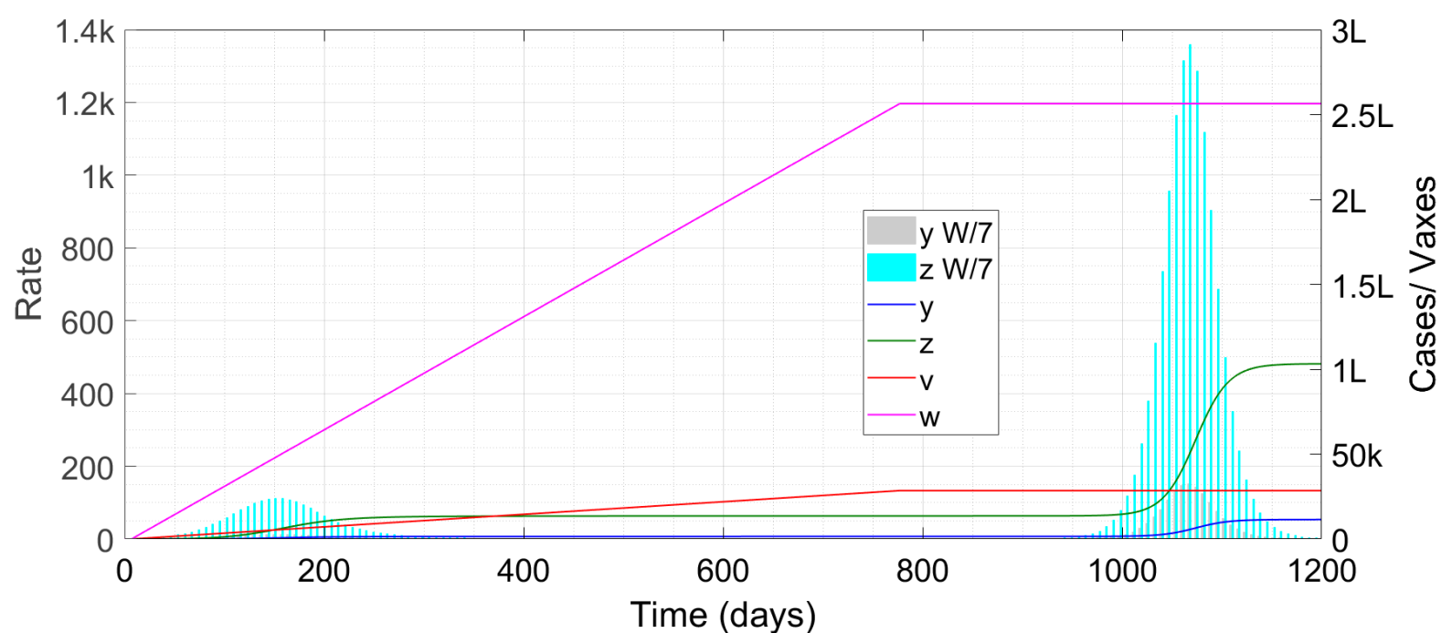
Figure 9 : Time trace of the epidemic with temporary immunity and vaccination rate just below the elimination cutoff. The symbol 'k' denotes thousand, 'L' hundred thousand and 'W/7' weekly cases scaled down by a factor of seven.
