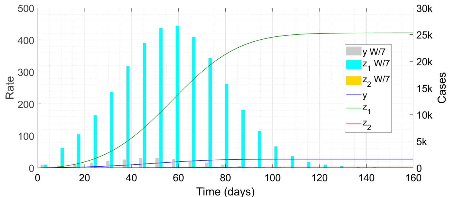
Figure 4 : Time trace of the epidemic with increased mobility for vaccinees. The symbol ‘k’ denotes thousand and ‘W/7’ weekly cases scaled down by a factor of seven.
