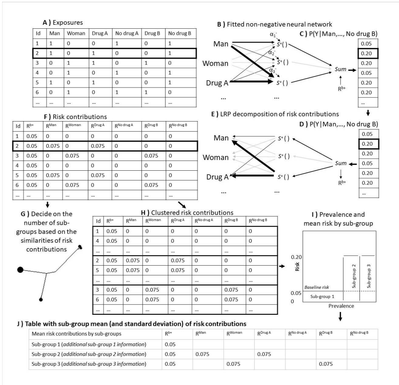
Figure 3. Workflow of the computational phase of CoOL
