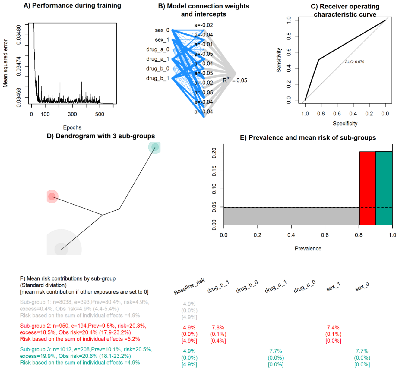
Figure 4. Results of the computational phase of CoOL
