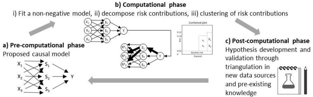
Figure 1. The phases of the CoOL approach towards inference to the best explanation
