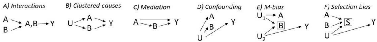
Figure 5. Six causal structures causing co-occurring associations
