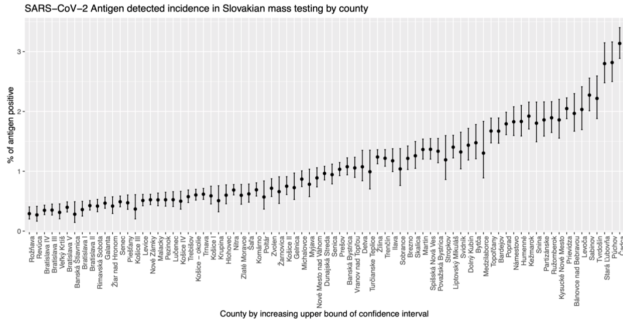
Figure 1: SARS-CoV-2 antigen detected incidence in Slovakian mass testing by county. Test positivity rates among the 3,625,332 tested persons in the 79 counties with simultaneous Bonferroni adjusted 95% confidence intervals. Counties are ordered from low to high incidence by the upper confidence bound. Data source [10].
