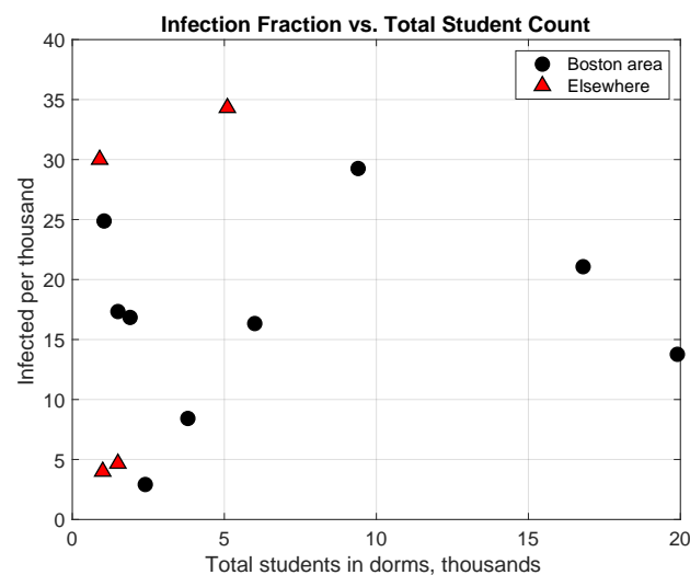
Fig. 1. Cumulative infected student fraction f vs. total students in residence. The vertical axis shows the total reported infections per thousand students. The horizontal axis is the total student dorm-residential population. Boston area schools are shown as circles, and comparison schools from other areas as triangles.
