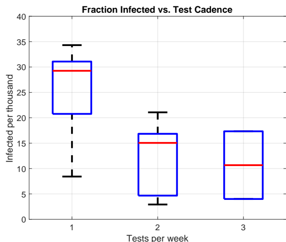
Fig. 4. Box plot of cumulative relative infection f as a function of PCR test cadence. There is evidence (p-value of 1.7%) that a campus testing frequency of more than once per week is correlated with lower f . There were only two institutions in our sample that carried out testing three times per week, so the horizontal bars of the blue box on the right correspond to those values, and the red bar is their mean.
