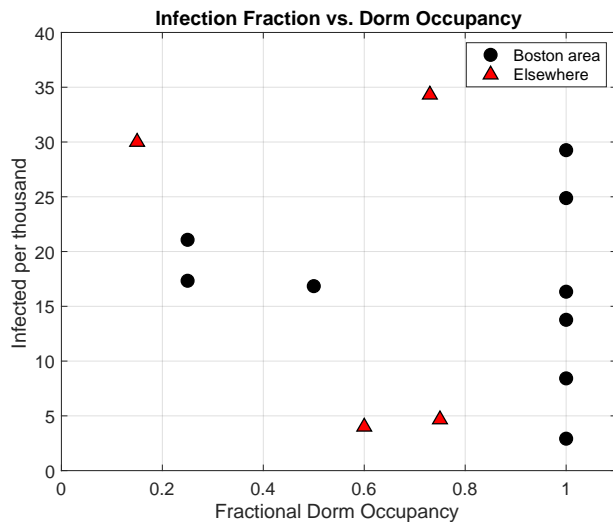
Fig. 2. Cumulative infected fraction f vs. dormitory density \rho . The vertical axis shows the total reported infection per thousand students. The horizontal axis is the dormitory residential density. Boston area schools are shown as circles, and comparison schools from other areas as triangles.
