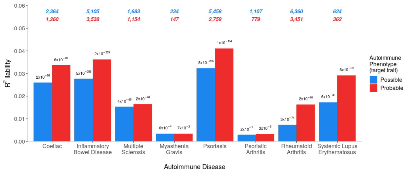
261 Figure 2: Variances in autoimmune liability explained by PRS for the corresponding autoimmune diseases. The number 262 of cases are shown at the top of the plot (possible = blue, probable = red). P-values are shown atop each bar.
