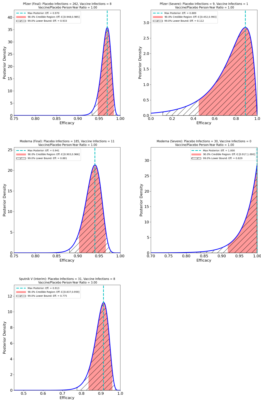
Figure 3.1: Efficacy estimates: Maximum a posteriori estimates (dashed line), 90% credible regions (solid shaded regions), and 99% lower bounds (hatched regions). Top: Pfizer/BioNTech, overall (left) and severe (right). Middle: Moderna overall (left) and severe (right). Bottom: Interim Sputnik V data.
