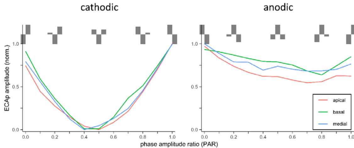
Figure 4. Median values of the normalized ECAP response amplitude collapsed across all participants for each electrode contact position (apical, medial, basal). Left side: p -triphasic pulses with cathodic second phase stimulated responses; right side: responses to pulses with anodic second phase.
