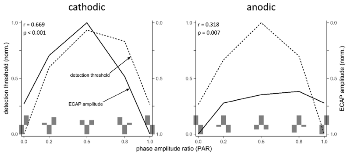
Figure 7: Median values of the inverted normalized ECAP response amplitudes (continuous line) and the normalized psychophysical detection thresholds (dashed line) of seven participants as functions of the tested PAR. Left side: results for p -triphasic pulses with cathodic second phase, right side: results for p -triphasic pulses with anodic second phase. Spearman's r and p -values in the upper right corner of each graph indicate the correlation and corresponding significance level of the correlation between both methods within each polarity.
