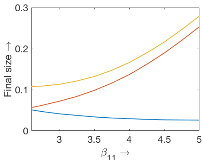
Figure 1: Final value of the total susceptible population and in the two sub-classes as functions of \beta_{11} , S_1^f - lower curve, S_2^f - middle curve, their sum - upper curve. The values of parameters: \beta_{22} = 5 - \beta_{11} , \beta_{12} = \beta_{21} = 2.5 , \sigma = 1 .
