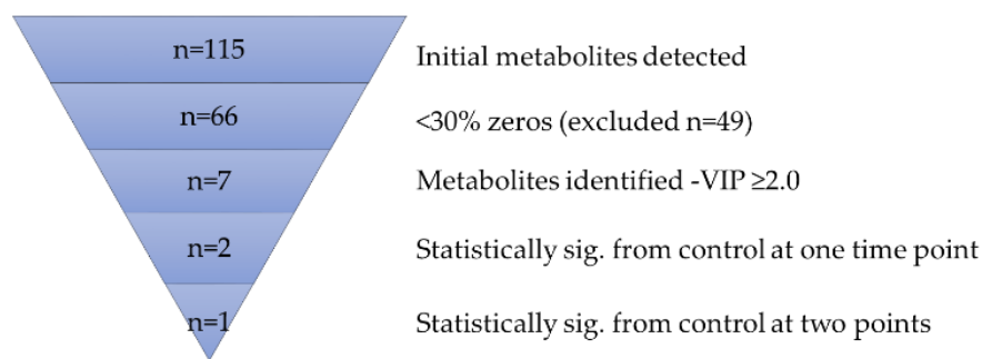
Figure 1: Overview-untargeted analysis
