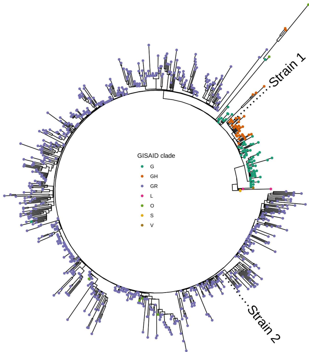
FIGURE 3. Phylogenetic tree of all of the available SARS-CoV-2 strains isolated in Russia (as of 11.11.2020). GISAID clade classification is represented by color. Tip labels mark positions of strain 1 (Russia/CRIE170668/2020, EPI_ISL_610237) and strain 2 (Russia/CRIE300223/2020, EPI_ISL_610238). Closely related to SARS-CoV-2 virus strain bat/Yunnan/RmYN02/2019 (EPI_ISL_412977) was used as a root (not shown).
