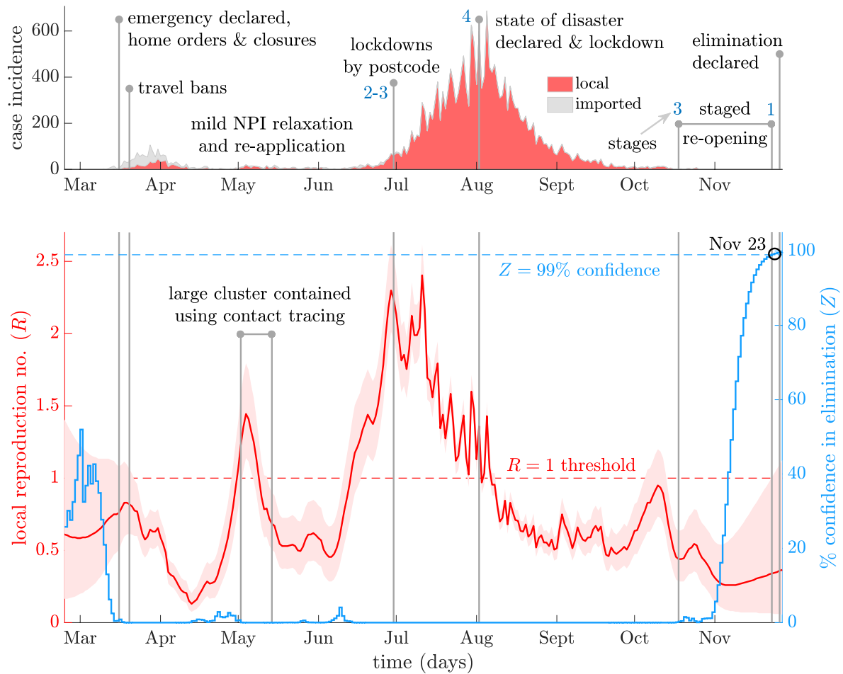
Figure 3: Local transmission dynamics of COVID-19 in Victoria, Australia. The top panel illustrates local (red) and imported (grey, stacked) cases by diagnosis date from (25). Vertical lines highlight important policy change-times and responses (blue numbers are NPI restriction stages). The bottom panel presents smoothed local R -estimates (red with 95% confidence bands) and resulting Z numbers (blue) measuring the % probability of elimination.
