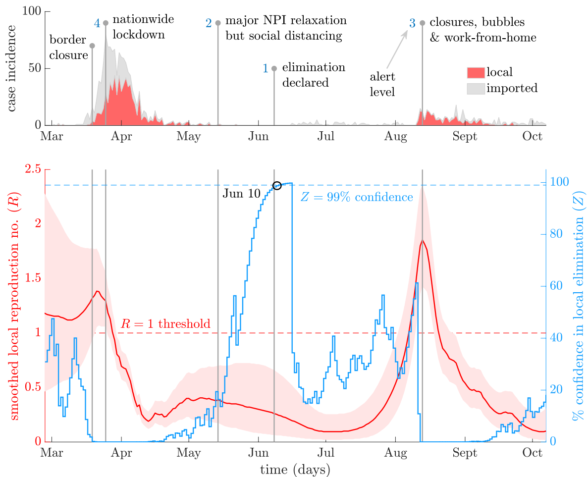
Figure 1: Local transmission dynamics of COVID-19 in New Zealand. The top panel plots local (red) and imported (grey, stacked) cases by date reported, sourced from (21). Vertical lines pinpoint key policy change-times and alert levels (blue numbers) in response to these caseloads. The bottom panel presents smoothed local R number estimates (red with 95% confidence bands) and Z numbers (blue), which measure % elimination potential.
