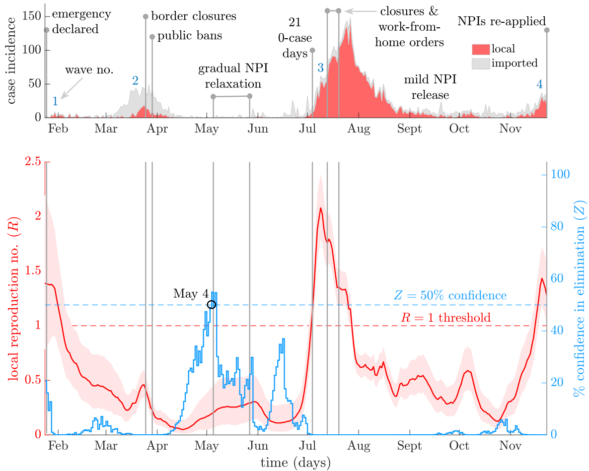
Figure 2: Local transmission dynamics of COVID-19 in Hong Kong, China. The top panel presents local cases (red) and imported cases (grey, stacked) by onset date from (6). Vertical lines demarcate key policy change-times and responses (blue numbers indicate waves). The bottom panel plots smoothed local R -estimates (red with 95% confidence bands) and associated Z numbers (blue) measuring the % likelihood of elimination.
