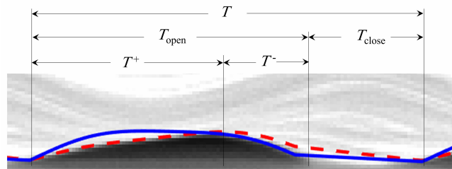
FIG. 5. (Color online) Kymogram at the mid anterior-posterior location of the VF model. Solid and dashed lines identify the sinusoidal functions that were respectively fitted to the inferior edge of the VF during closure, and the superior edge during opening, via least-squares regression 66 .
