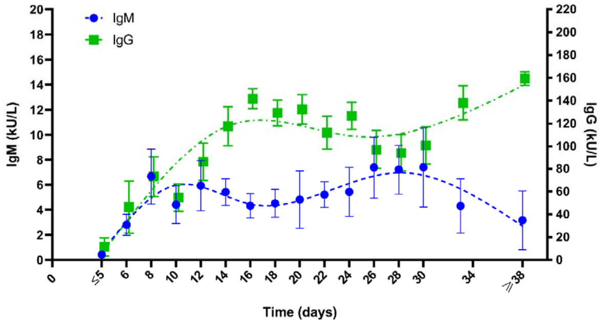
Figure 3: Time kinetic results of Mindray SARS-CoV-2 IgM and IgG results. In this study, a series of 44 COVID-19 positive patients (at nasopharyngeal rRT-PCR test) were included and followed-up. Mean and Standard errors are reported. Spline regressions (with 4 points knots) were used to generate the time-kinetic trends.
