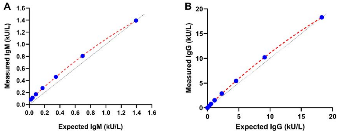
Figure 1: IgM and IgG antibody assay linearity results. For IgM, a high-level pool at 1.4 kU/L was serially diluted with a low-level pool at 0.01 kU/L. For IgG, a high-level pool at 18.70 kU/L was serially diluted with a low-level pool at 0.5 kU/L. Averages of triplicate measurements are shown. Second order polynomial interpolation reported a significant deviation from linearity for both IgM and IgG.
