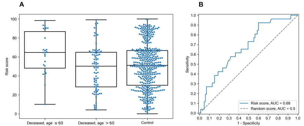
Fig 4. Risk score (RS) separates groups of adult and elderly patients. A: distribution of RS in adult, elderly and control patient groups. B: receiver operating characteristic curve for RS separating patients from adult and elderly groups.
