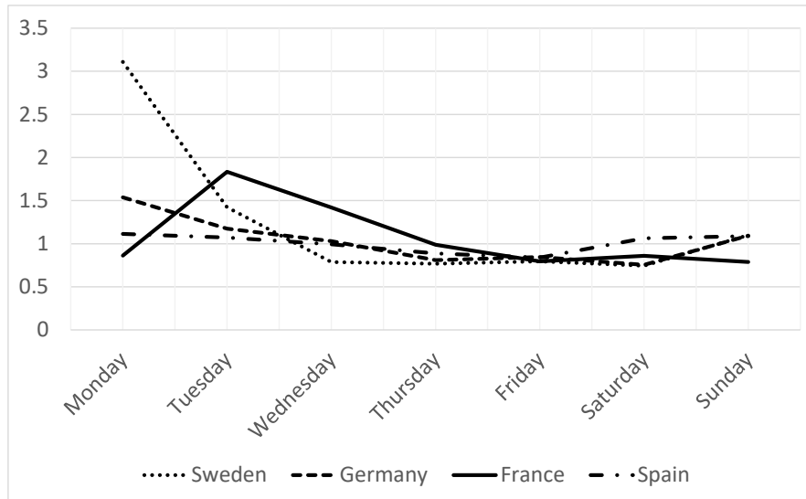
Figure 2: Plot of \hat{\mathbf{q}}(i, \hat{R}, \Phi) = (\hat{q}_0, \hat{q}_1, \hat{q}_2, \hat{q}_3, \hat{q}_4, \hat{q}_5, \hat{q}_6) for different countries.
