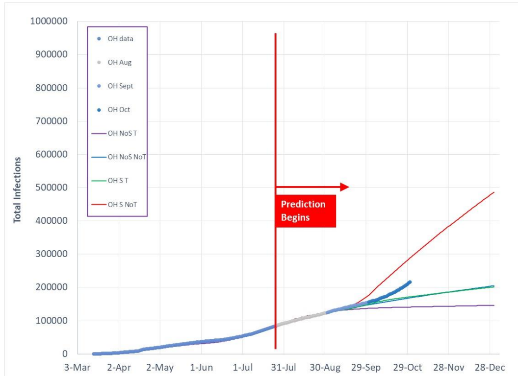
Figure 11 Total Covid-19 infection predictions as of July 27, 2020 for 4 model cases in comparison to actual data for OH.
