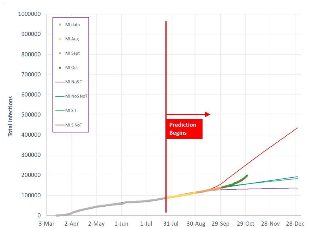
Figure 12 Total Covid-19 infection predictions as of July 27, 2020 for 4 model cases in comparison to actual data for MI.
