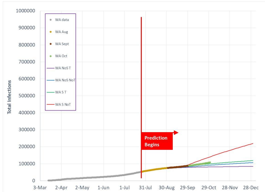
Figure 15 Total Covid-19 infection predictions as of July 27, 2020 for 4 model cases in comparison to actual data for WA.
