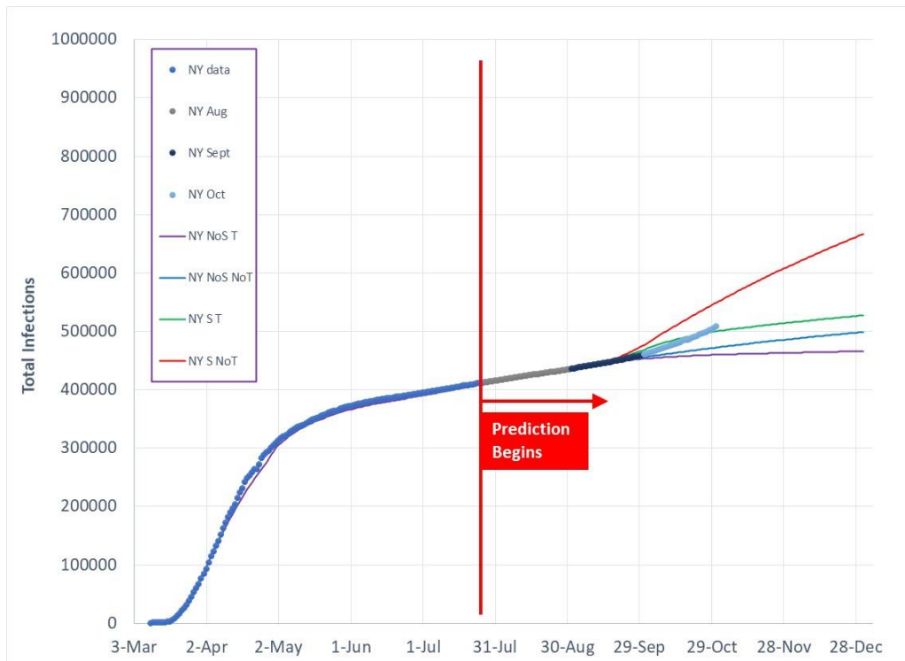
Figure 6 Total Covid-19 infection predictions as of July 27, 2020 for 4 model cases in comparison to actual data for NY.
