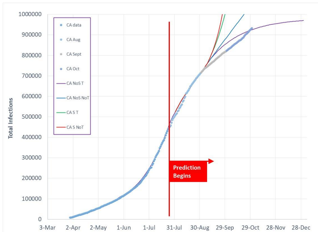
Figure 14 Total Covid-19 infection predictions as of July 27, 2020 for 4 model cases in comparison to actual data for CA.
