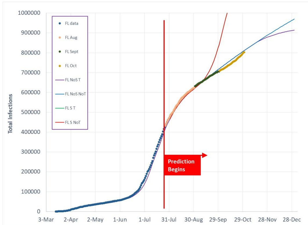
Figure 13 Total Covid-19 infection predictions as of July 27, 2020 for 4 model cases in comparison to actual data for FL.
