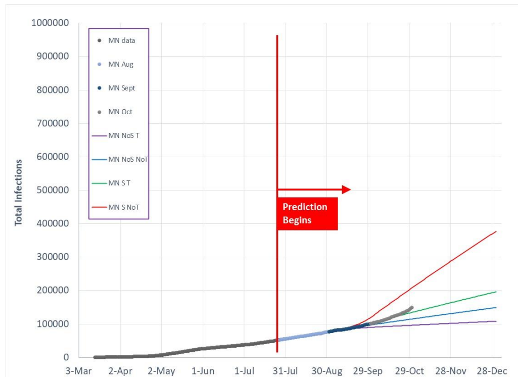
Figure 10 Total Covid-19 infection predictions as of July 27, 2020 for 4 model cases in comparison to actual data for MN.
