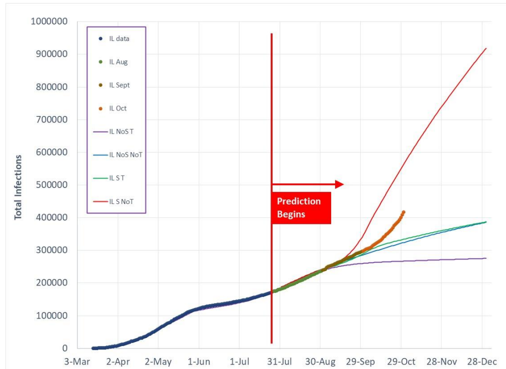
Figure 9 Total Covid-19 infection predictions as of July 27, 2020 for 4 model cases in comparison to actual data for IL.
