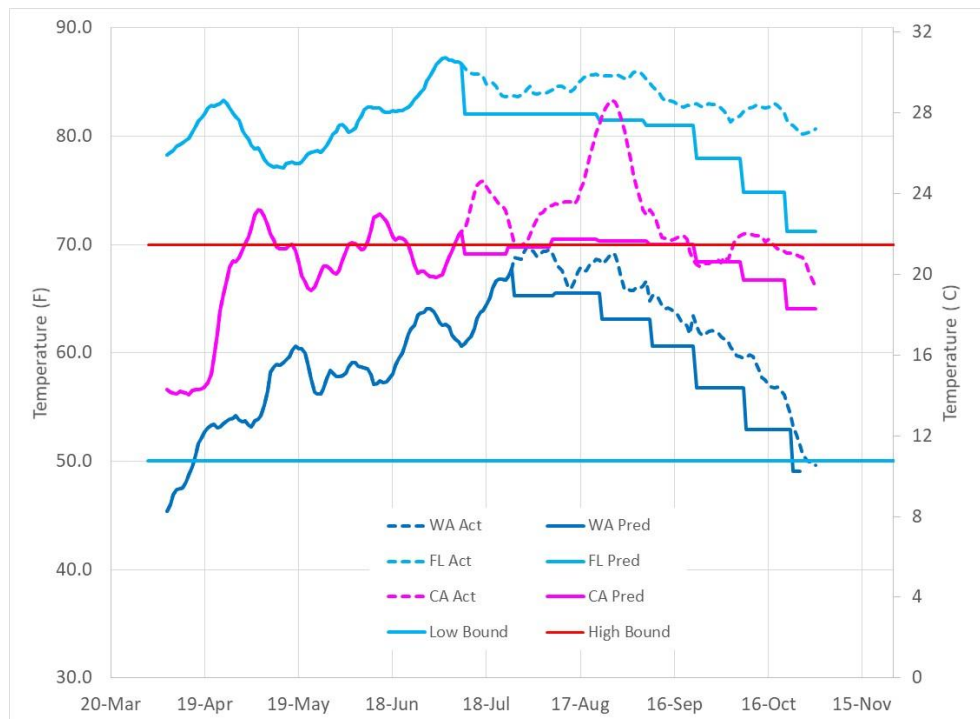
Figure 4 Historical average outdoor temperatures and actual average outdoor temperatures for FL, CA, and WA.
