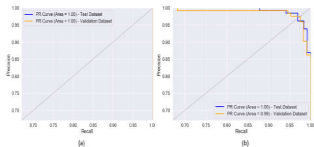
Fig. 7. Precision-Recall curves for the class: (a) COVID-19 (b) Viral Pneumonia
