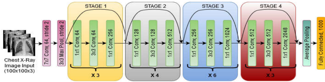
Fig. 3. Structure of ResNet-50 for the classification of COVID-19 from chest X-ray images
