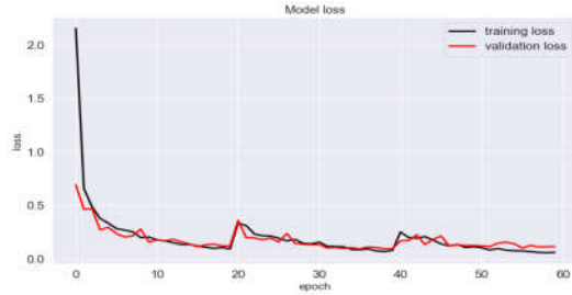
Fig. 11. Loss between training and validation by ResNet-50 model
