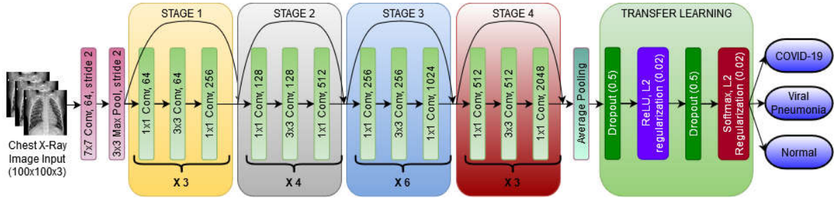
Fig. 4. Proposed deep transfer learning on the ResNet-50 for the classification of COVID-19 from chest X-ray images
