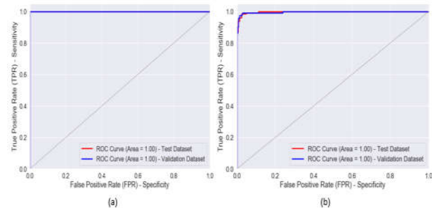
Fig. 9. ROC curves representing the class: (a) COVID-19 (b) Viral Pneumonia
