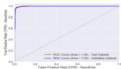
Fig. 10. ROC curves representing the class NORMAL
