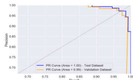
Fig. 8. Precision-Recall curve for the class NORMAL
