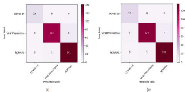
Fig. 5. Confusion matrix of the proposed model: (a) test set (b) validation set
