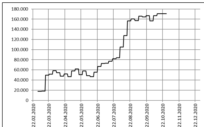
Fig. 4. Daily test volume T_k (weekly reports by RKI)
