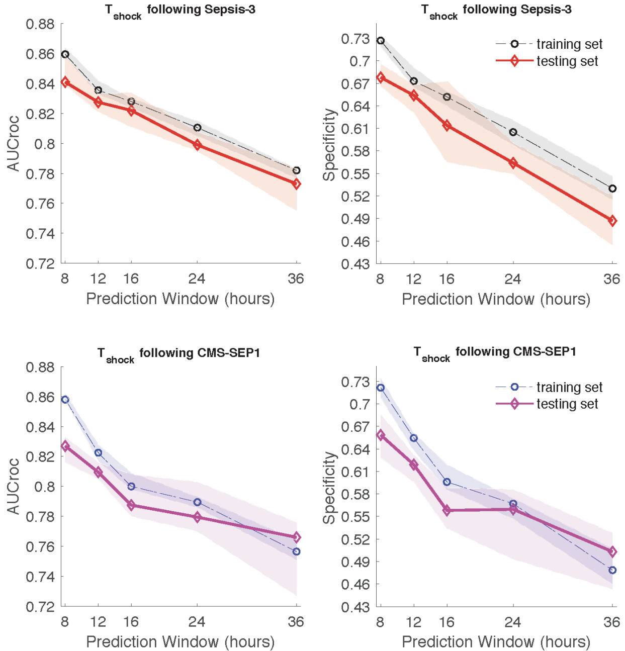
507 Figure 3: Comparison of AUC and specificity (calculated at 85% sensitivity) of models predicting 508 septic shock at different prediction windows at the validation site. 10-fold cross-validation was 509 performed and a median and inter-quartiles are presented using lines and shaded areas, 510 respectively.
