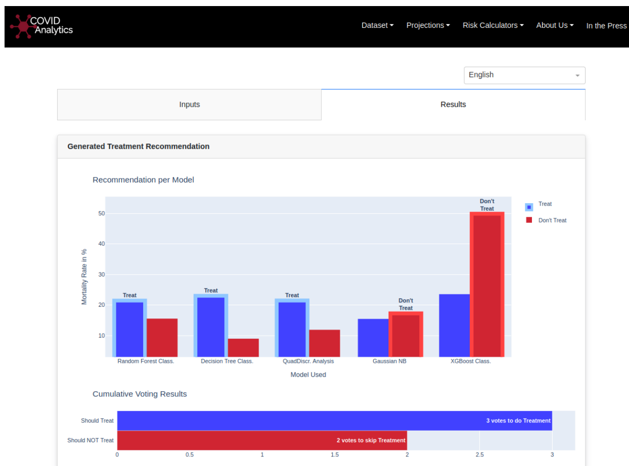
Fig. 4: Visualization of the online algorithm user interface.
