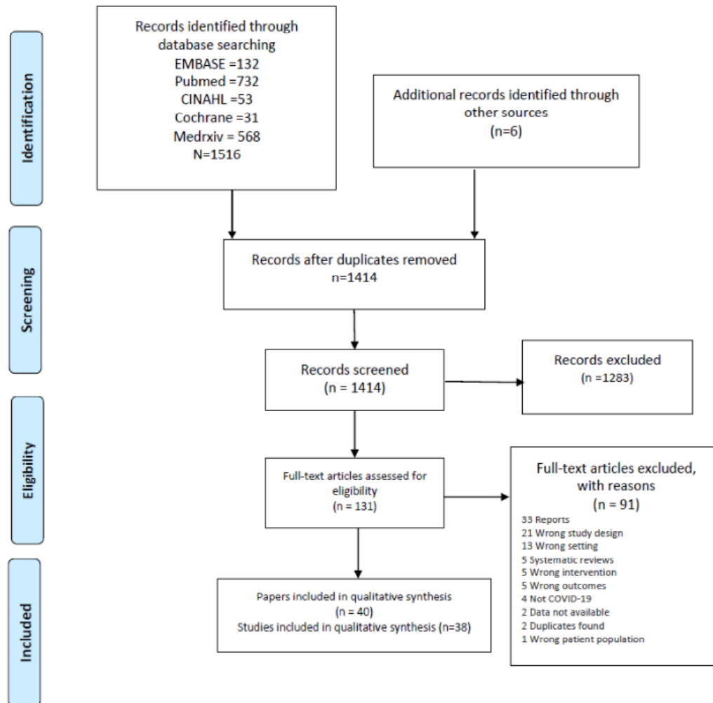
Figure 1 PRISMA Flowchart
