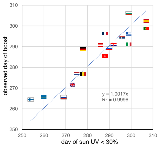
91 Figure 4: observed day of the second wave covid-19 boost as a function of the day when the country 92 sun UV daily dose drops lower than 30% of that at latitude 0°. Trendline forced to intercept (0,0).
