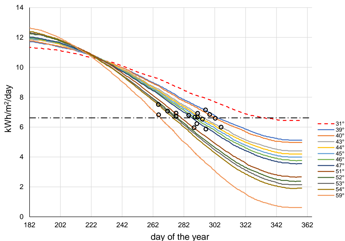
Figure 3: Solid curves: theoretical total daily sun insolation under a clear sky corresponding to the 14 PWC country latitudes. Black circles: country boost dates positioned on their corresponding latitude curve. Black dot-dash line corresponds to the average sun irradiance threshold, i.e. \approx 7 \text{ kWh/m}^2/\text{day} .
