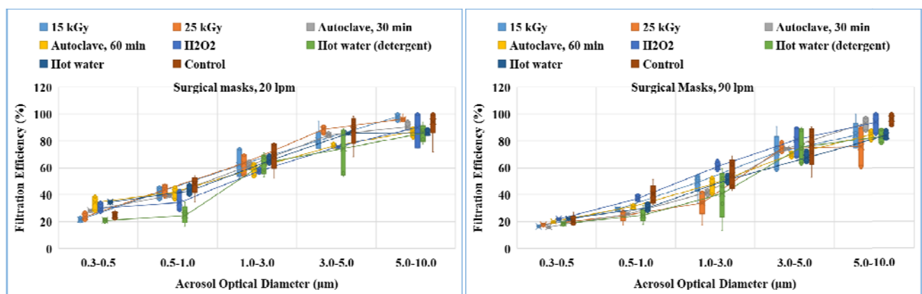
Fig. 8. FE of surgical equivalent face masks after gamma, autoclave, \text{H}_2\text{O}_2 sterilization and hot water with and without detergent sterilization for 20 and 90 lpm flow rates.
