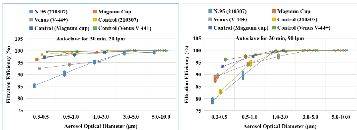
Fig. 7. FE of various certified N-95 facemasks after autoclave sterilization for 20 and 90 lpm flow rates.
