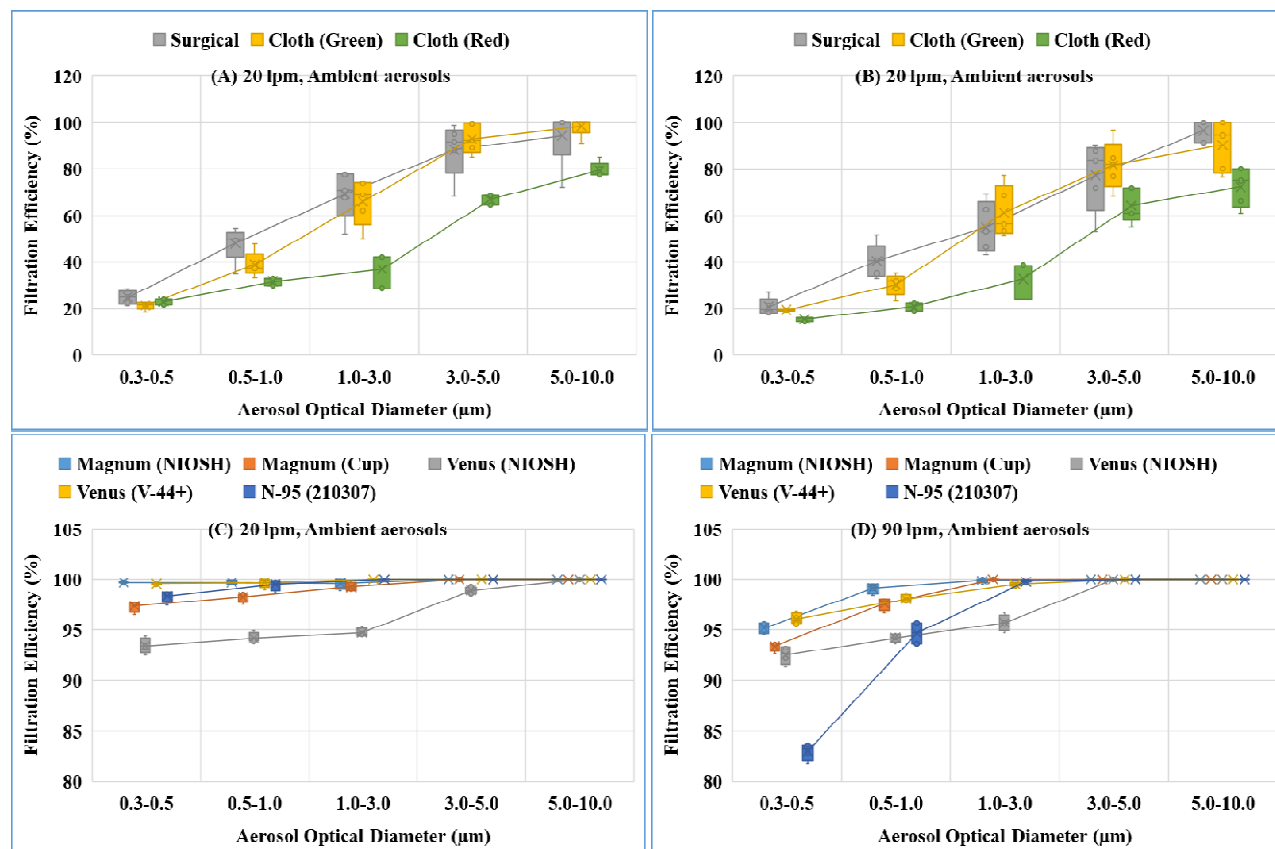
Fig. 4. FE of individual control facemasks at a flow rate 20 and 90 lpm for ambient aerosols. (A) and (B) cloth and surgical facemasks (C) and (D) different type certified N-95 facemasks.
