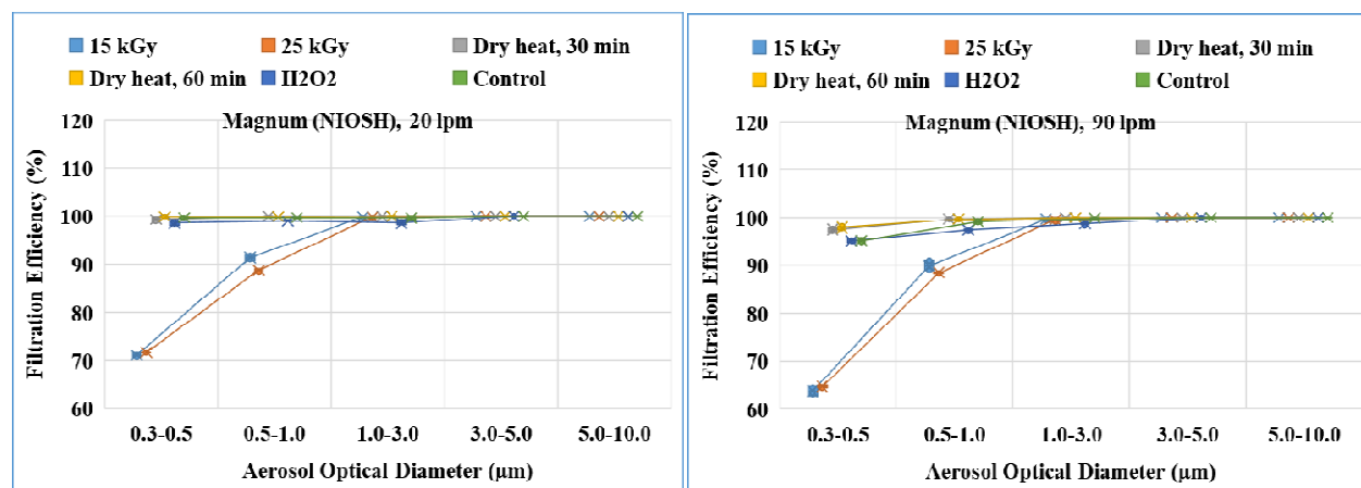
Fig. 5. FE of N-95 (Magnum NIOSH) face masks after gamma, dry heat and H 2 O 2 sterilization for 20 and 90 lpm flow rates.
