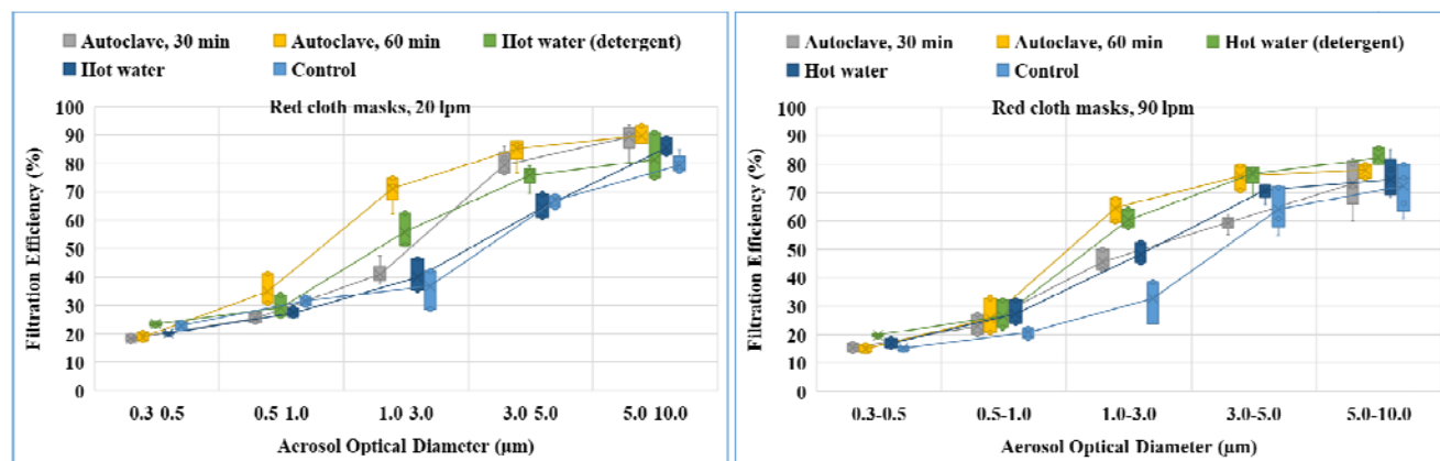
Fig. 10. FE of double layer (red cloth different fabric) face masks after autoclave, hot water with and without detergent sterilization for 20 and 90 lpm flow rates.
