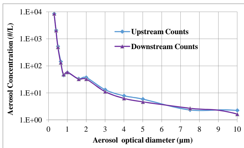
Fig. 2. Upstream and downstream average aerosols counts as a function of optical diameter measured by OPC.
