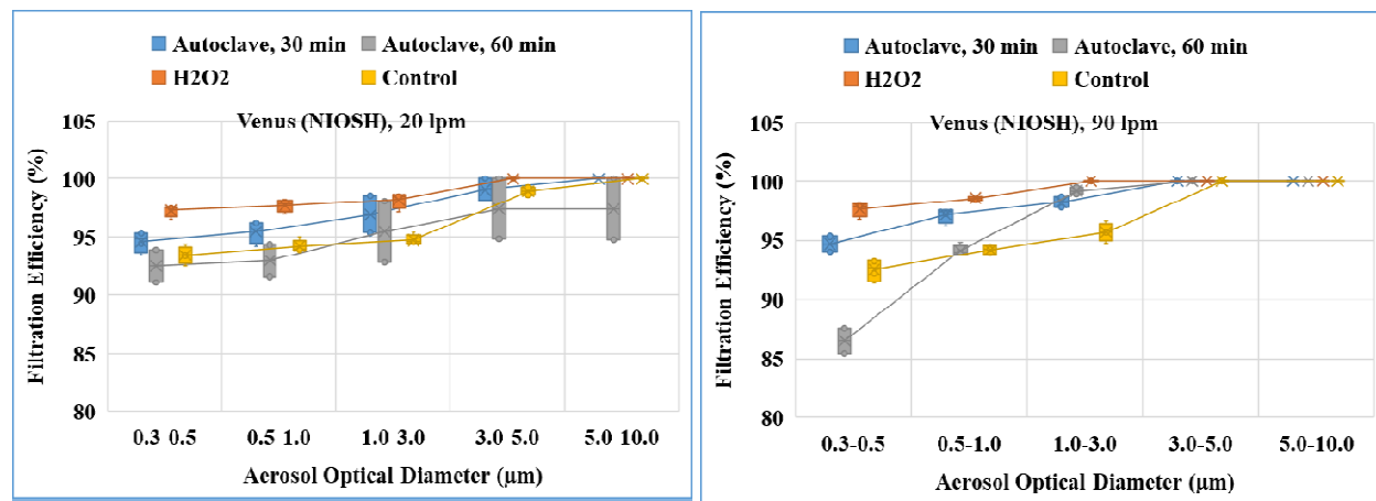
Fig.6. FE of N-95 (Venus NIOSH) face masks after autoclave and H 2 O 2 sterilization for 20 and 90 lpm flow rates.
