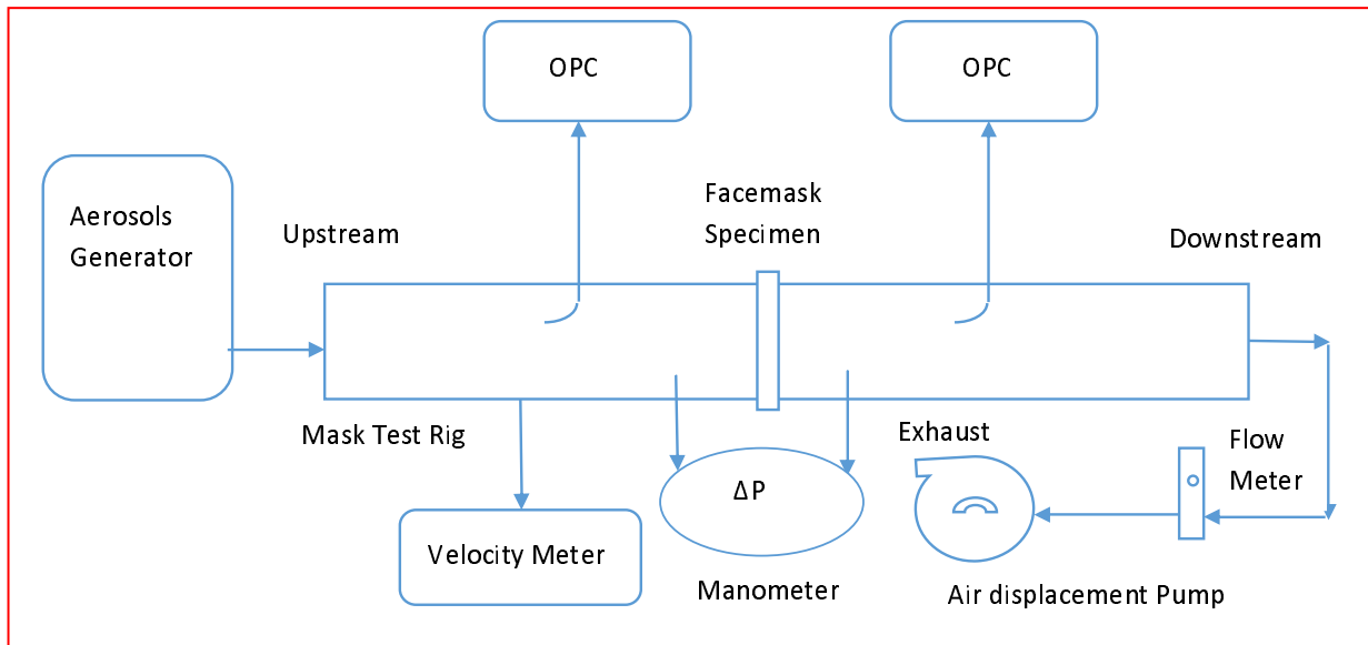
Fig. 1. Schematic presentation of experimental setup.
