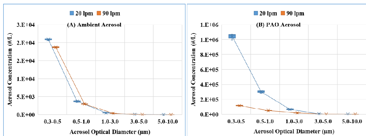
Fig.3. Aerosols concentration as a function of optical diameter of aerosols at a two flow rates, ambient (A) and PAO (B) aerosols.
