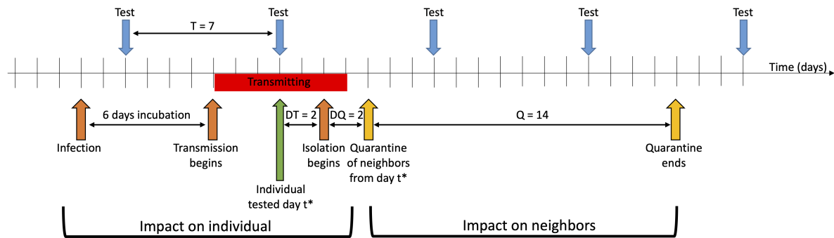
Figure 3. Schematic for the proposed mitigation strategy. Vertical arrows indicate various external actions on the population. The frequency of these control measures and the time delays between the different interventions represent the crucial control parameters for containing the infection. In this schematic, we show the standard value of parameters found in Table 1.
