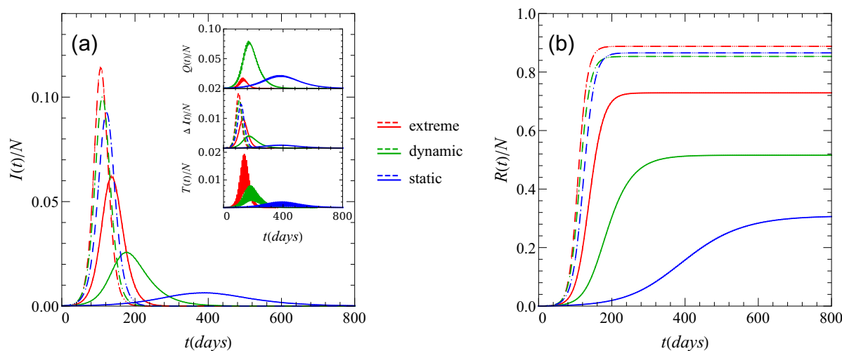
Figure 4. Mitigated and unmitigated time evolution of (a) the fraction of infectious and (b) recovered individuals for three different choices of the underlying network. The insets additionally display the fractions: T(t)/N of isolated individuals, \Delta I(t)/N of daily new infections, and Q(t)/N of quarantined individuals. For all mitigated curves we used the standard values of the mitigation parameters that are shown in Table 1. The dashed curves correspond to unmitigated dynamics.
