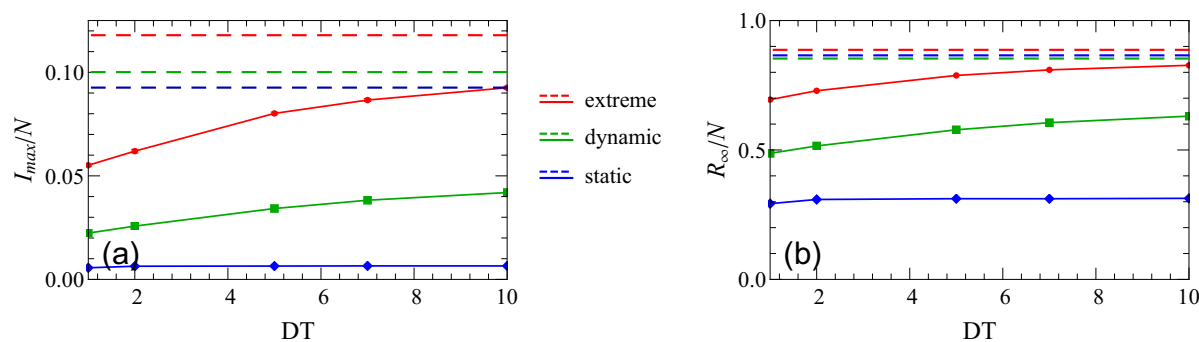
Figure 7. Change of (a) the peak of the infectious curve I_{max}/N and (b) the fraction of total recovered population R_{\infty}/N with the delay to testing DT for different setups. The other mitigation parameters are set to their default values ( f = 0.5 , TP = 7 , DQ = 2 , Q = 14 ). The dashed lines represent unmitigated scenarios.
