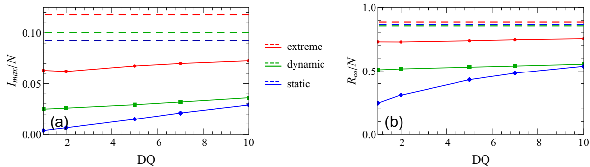
Figure 9. Change of (a) the peak of the infectious curve I_{max}/N and (b) the fraction of total recovered population R_{\infty}/N with the delay to quarantine for different setups. The other mitigation parameters are set to their default values ( f = 0.5 , TP = 7 , DT = 2 , Q = 14 ). The dashed lines represent unmitigated scenarios.
