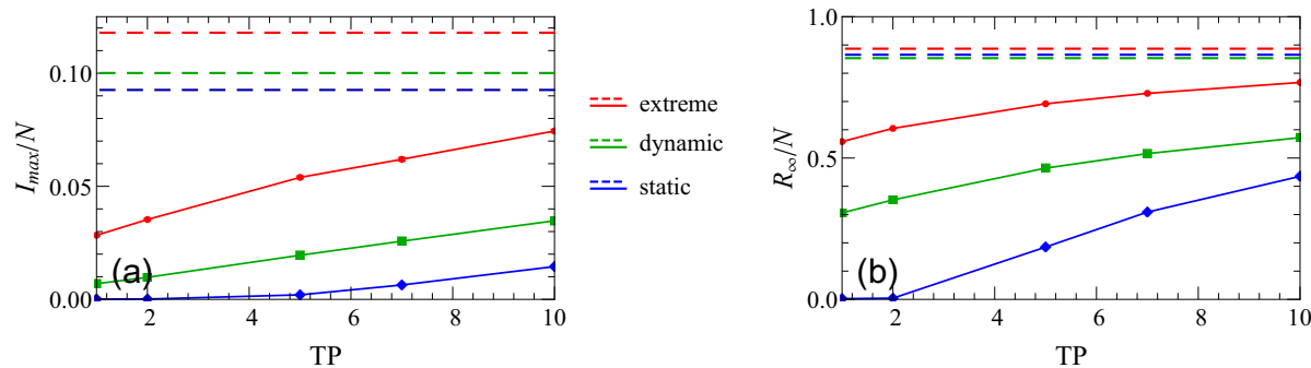
Figure 6. Change of (a) the peak of the infectious curve I_{max}/N and (b) the fraction of total recovered population R_{\infty}/N with the testing period TP for different setups. The other mitigation parameters are set to their default values ( f = 0.5 , DT = 2 , DQ = 2 , Q = 14 ). The dashed lines represent unmitigated scenarios.
