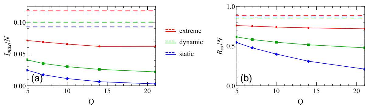
Figure 8. Change of (a) the peak of the infectious curve I_{max}/N and (b) the fraction of total recovered population R_{\infty}/N with the quarantine duration for different setups. The other mitigation parameters are set to their default values ( f = 0.5 , TP = 7 , DT = 2 , DQ = 2 ). The dashed lines represent unmitigated scenarios.
