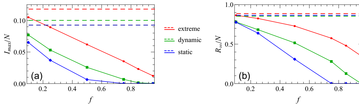
Figure 5. Change of (a) the peak of the infectious curve I_{max}/N and (b) the fraction of total recovered population R_{\infty}/N with the fraction of identified infectious individuals f for three different setups. The other mitigation parameters are set to their default values (TP = 7, DT = 2, DQ = 2, Q = 14). The dashed lines represent unmitigated scenarios.
