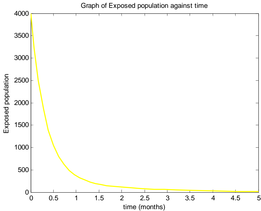
Fig(3), is the graph of exposed population against time, from the graph, the exposed population decreases as time increases, the exposed population decreases to zero indicating that with time the COVID-19 pandemic can be controlled in Nigeria since the exposed population tends to zero.
