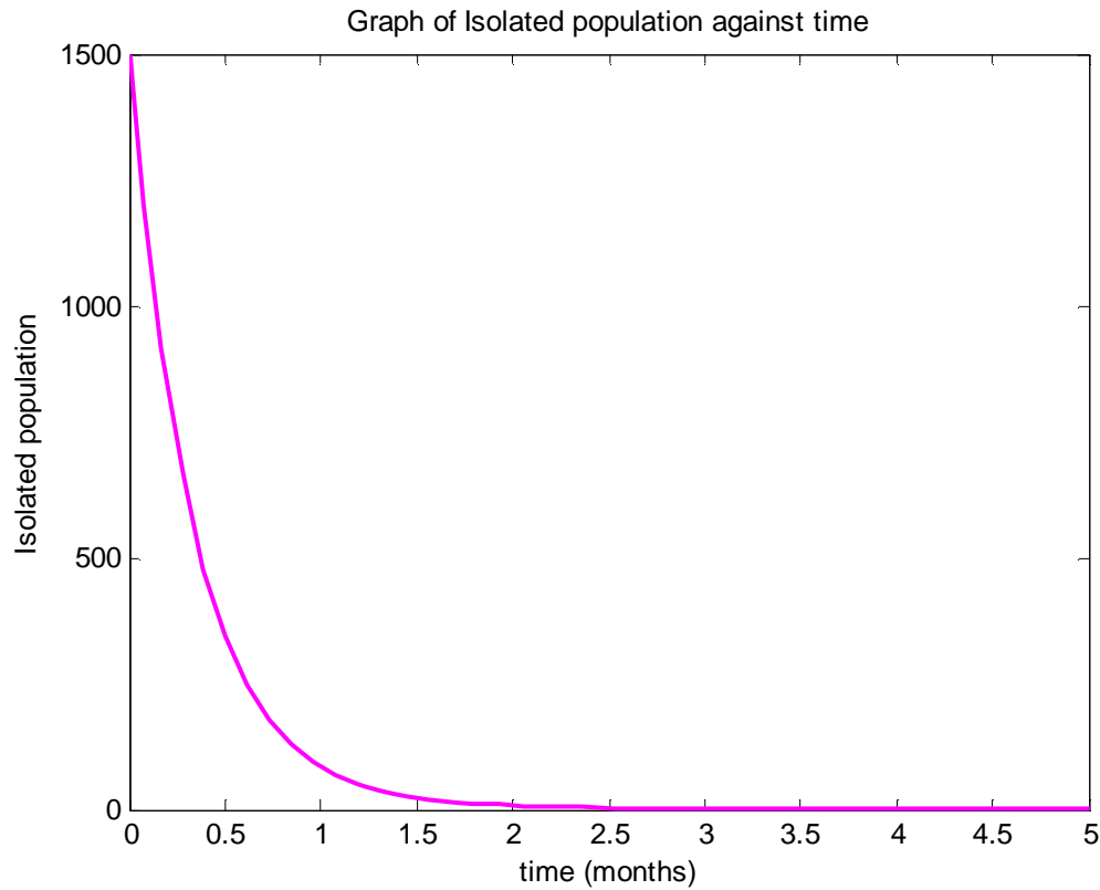
Fig(6), is the graph of isolated population against time, it is observed that isolated population decreases in Nigeria as time increases this could be as a result of decrease in infected population and rapid increase of recovered individuals.
