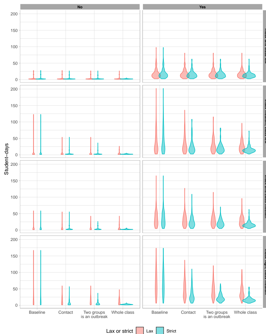
Fig 5. Asymptomatic student-days: the number of student-days on which a student is infectious but not yet told to isolate. Left: index case is symptomatic. Right: index case is asymptomatic. Lax: Only symptomatic students are ever told to isolate. Strict: All student in a shut down group or class are told to isolate.
