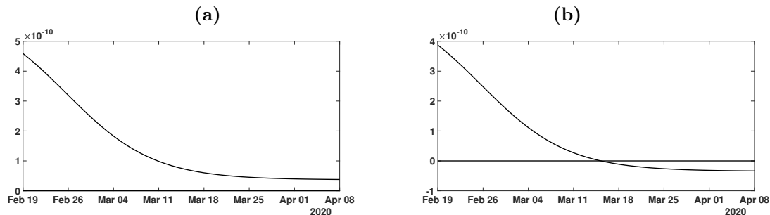
Figure 4: In this figure, we plot the rate of transmission obtained from formula (4.5) with f = 0.5 , \chi_2 \theta = 0.14 < \nu = 0.2 (in Figure (a)) and \nu = 0.1 < \chi_2 \theta = 0.14 (in Figure (b)), \chi_2 = 0.66 and \theta = 0.22 and CR_\infty = 67102 which is the latest value obtained from the cumulative number of reported cases for China.
