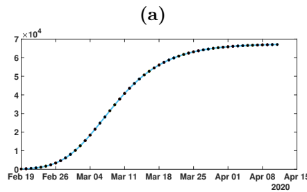
Figure 6: In this figure, we plot the perfect fit of the cumulative number of reported cases of COVID-19 in China. We fix the parameters f = 0.5 and \nu = 0.2 or \nu = 0.1 and we apply our algorithm 1 to obtain the perfect fit. The black dots correspond to data for the cumulative number of reported cases obtain and the blue curve corresponds to the model.
