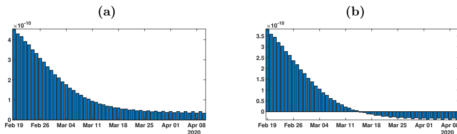
Figure 7: In this figure, we plot the rate of transmission obtained for the reported cases of COVID-19 in China with the parameters f = 0.5 and \nu = 0.2 in figure (a) and \nu = 0.1 in figure (b). This rate of transmission corresponds to the perfect fit obtained in Figure 6.
