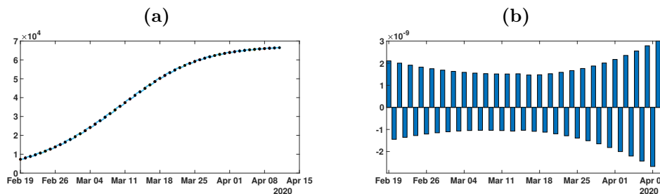
Figure 10: We apply Algorithm 1 the regularized data. In figure (a), we plot the regularized cumulative number of reported cases obtained from the data (black dots) and the model (blue curve). In figure (b), we plot the daily rate of transmission obtained by using Algorithm 1. We see that we can fit the data perfectly. But the method is very unstable. We obtain a rate of transmission that oscillates from the positive to the negative value back and forth.
