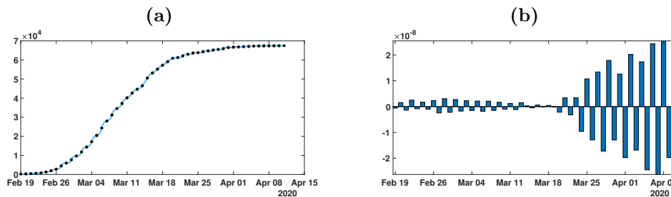
Figure 9: In figure (a), we plot the cumulative number of reported cases obtained from the data (black dots) and the model (blue curve). In figure (b), we plot the daily rate of transmission obtained by using Algorithm 1. We see that we can fit the data perfectly. But the method being very unstable. We obtain a rate of transmission that oscillates from the positive to the negative value back and forth.
