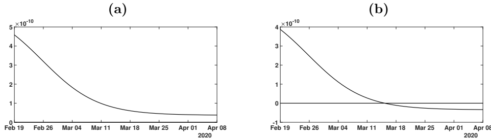
Figure 4: In this figure, we plot the rate of transmission obtained from formula (4.5) with f = 0.5 , \nu = 0.2 (in Figure (a)) and \nu = 0.1 (in Figure (b)), \chi_2 = 0.66 and \theta = 0.22 (i.e. \chi_2\theta = 0.14 < \nu ) and CR_\infty = 67102 which is the latest value obtained from the cumulative number of reported cases for China.
