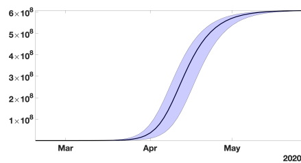
Figure 2: In this figure, the black curve corresponds to the cumulative number of reported cases CR(t) obtained from the model (2.6) with CR'(t) = \nu f I(t) by using the values I_0 = 1521 and \tau_0 = 3.32 \times 10^{-10} obtained from our method and the early data from February 19 to March 1. The blue region corresponds the 95% confidence interval when the rate of transmission \tau(t) is constant and equal to the estimated value \tau_0 = 3.32 \times 10^{-10} .
