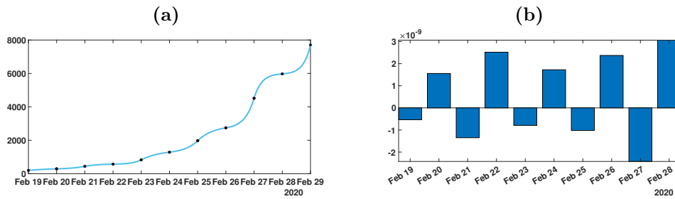
Figure 8: In figure (a), we plot the cumulative number of reported cases obtained from the data (black dots) and the model (blue curve). In figure (b), we plot the daily rate of transmission obtained by using Algorithm 1. We see that we can fit the data perfectly. But the method is very unstable. We obtain a rate of transmission that oscillates from the positive to the negative value back and forth.
