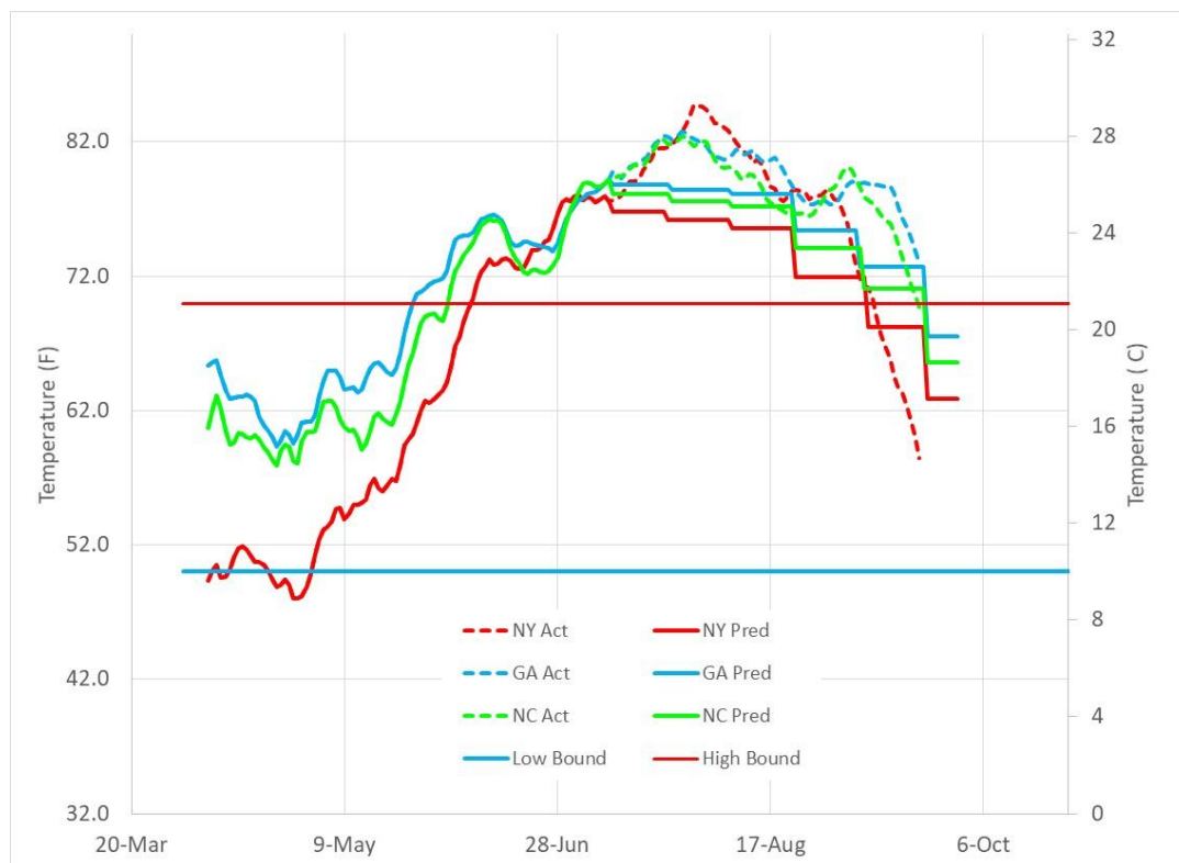
Figure 1 Historical average outdoor temperatures and September 2020 average outdoor temperatures for NY, NC and GA.
